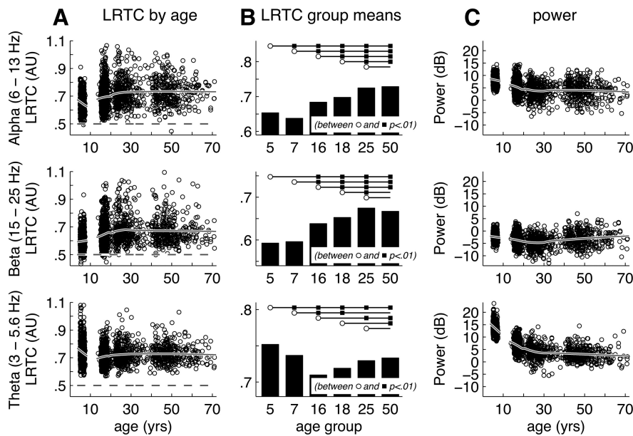
Figure 2. LRTC exhibit prolonged development for all oscillation frequencies. LRTC and EEG power development for alpha (top row)-, beta (middle row)-, and theta (bottom row)-oscillations. Data for a typical region (right central C4) are shown. A , The developmental profile of LRTC is fitted with a loess smooth (linear, 37% window size) and shown superposed on the DFA exponents of individual subjects ( n = 1433 ). LRTC for all three oscillation frequencies showed a steady increase from childhood up to adulthood reaching a plateau between 25 and 30 years. B , Age-group averages showed significant increases in LRTC from childhood to adolescence and adolescence to adulthood. Especially the alpha band oscillations showed significant increase between nearly all age groups (except between 5 and 7 years and 25 and 50 years), suggesting that LRTC reflect prolonged brain maturation in the third decade of life. C , Power showed developmental trends opposite to that of LRTC, which indicates that changes in LRTC cannot be explained by changes in signal-to-noise ratio. However, the decimation of EEG power (a 10 dB decrease) from childhood to adolescence may explain the strong decrease in theta LRTC.
