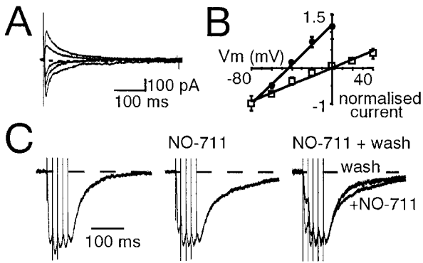
Figure 4. A , Synaptic currents recorded in the presence of 10 \mu\text{M} bicuculline at membrane potentials of -60 , -40 , -20 , 0 , and +10 mV using low-chloride internal solution. B , Normalized current–voltage relationship for IPSCs recorded in 10 \mu\text{M} bicuculline using low-chloride (closed circles) ( n = 4 ) and high-chloride internal solutions (open squares) ( n = 6 ). The reversal potential in low-chloride internal was -44 mV, whereas in high-internal chloride it was 0 mV. C , The GABA uptake blocker NO-711 slows the decay of the synaptic current; after washout of NO-711, the decay returns back to the control response.
