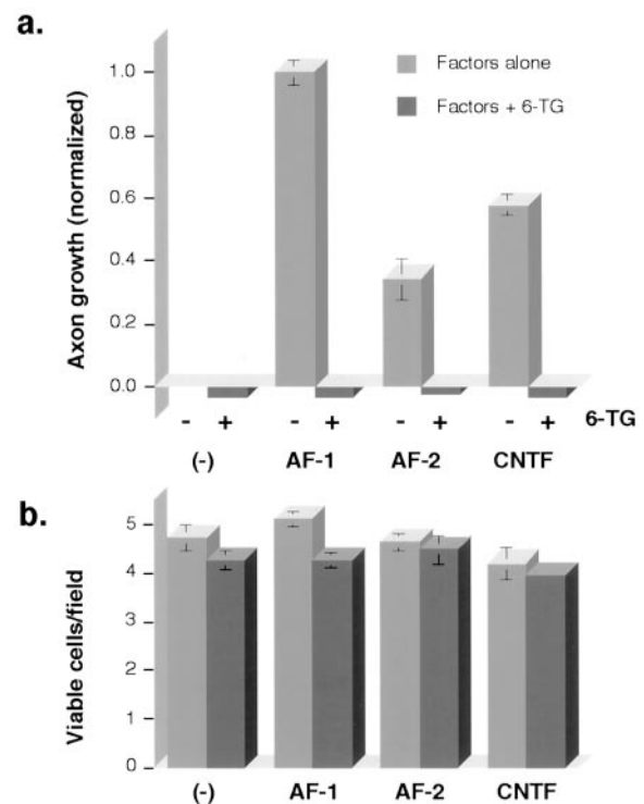
Figure 3. The purine analog 6-TG blocks neurite outgrowth induced by all three growth factors. a , Lightly shaded bars indicate growth induced by saturating concentrations of AF-1, AF-2, or CNTF. In the presence of 6-TG (20 \mu M), all growth was reduced below baseline (darkly shaded bars). b , 6-TG does not diminish cell survival (shown as the number of viable gRGCs per 400 \times microscope field, averaged over 20–30 fields per well and 4 wells per condition).
