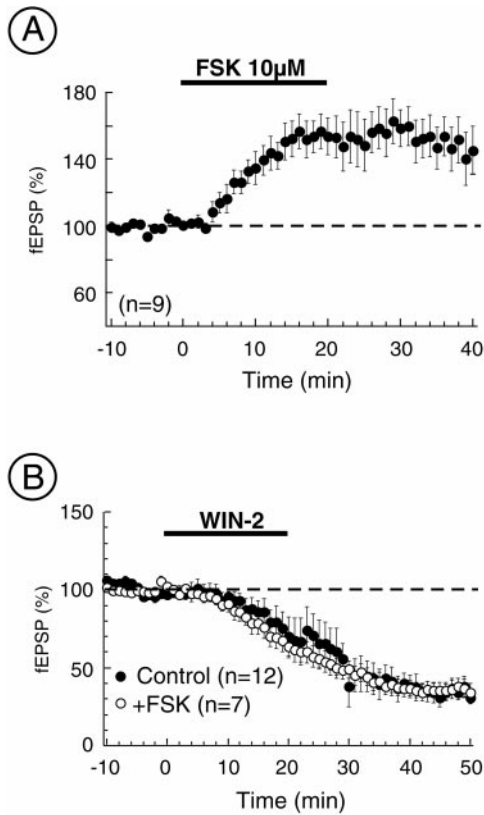
Figure 5. CB1-mediated inhibition is independent of cAMP levels. A , The adenylate cyclase activator forskolin (FSK; 10 \mu M, 20 min) caused a robust augmentation of the fEPSP in NAc slices ( n = 9 ). B , The WIN-2-mediated fEPSP inhibition was not affected when cAMP levels were augmented by bath application of forskolin ( n = 7 ). Forskolin was applied 20 min before and during the WIN-2 application (10 \mu M).
