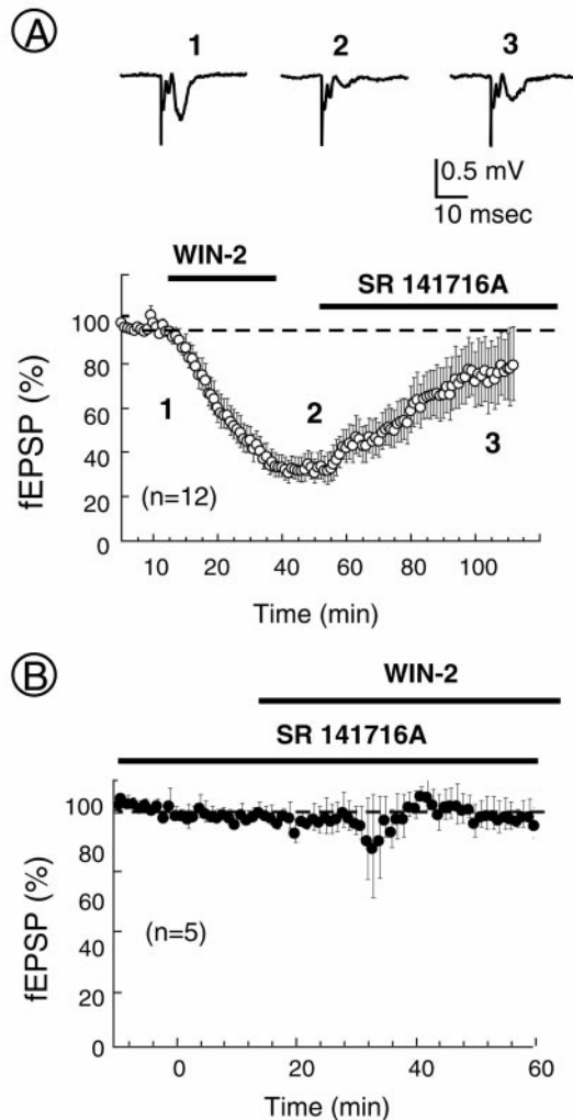
Figure 2. CB1 receptor-mediated inhibition of evoked excitatory synaptic transmission in mice nucleus accumbens. A , The cannabimimetic WIN-2 ( 10 \mu\text{M} ) reduced the fEPSP on average to 34 \pm 5\% ( n = 12 ) of its basal value. Traces represent averages of 10 consecutive EPSPs. The effects of WIN-2 were reversed by the selective CB1 antagonist SR 141716A ( 10 \mu\text{M} ). B , Preincubation of the slices with 10 \mu\text{M} of the CB1 antagonist SR 141716A was without effect on basal synaptic transmission (data not shown) but completely prevented the WIN-2-induced inhibition ( n = 5 ).
