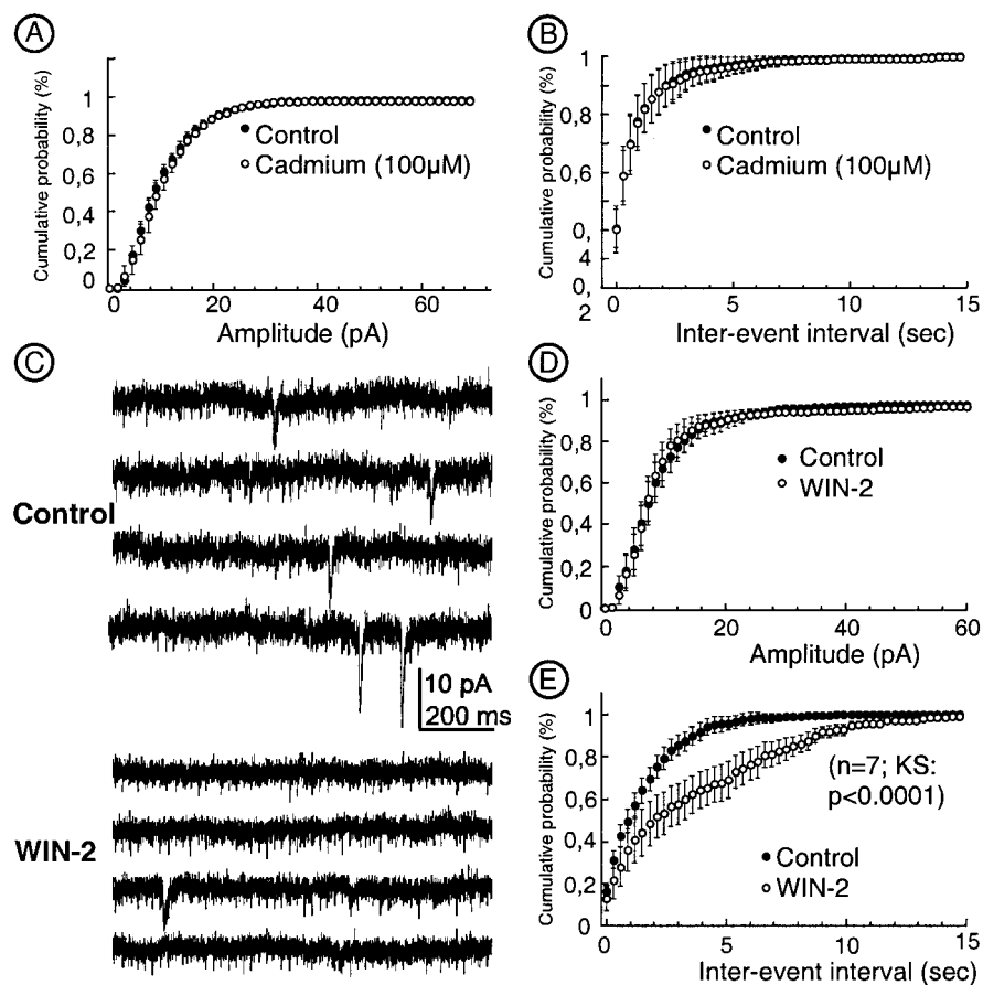
Figure 4. CB1-induced inhibition of action potential-independent glutamate release reveals a presynaptic site of action. A, B , Miniature EPSCs recorded in the presence of TTX are independent of Ca^{2+} channels activation. Bath application of cadmium chloride ( 100 \mu M ) to block voltage-sensitive Ca^{2+} channels changed neither the amplitude distribution ( A ) nor the frequency distribution of mEPSCs ( B ). C , Representative consecutive 1 sec current sweeps from a cell (holding potential of -70 mV) in which mEPSCs were recorded in the absence or presence of 10 \mu M WIN-2. D , The distribution of mEPSC amplitude before and during the application of the CB1 agonist, in the seven cells recorded, was unchanged after 20 min bath perfusion of WIN-2. E , The distribution of the time intervals between successive mEPSCs in all of the neurons recorded (same as above) revealed that the mEPSCs frequency was reduced during WIN-2 application. For control conditions, a total of 1849 events were detected over a period of 9.14 \pm 1.14 min ( n = 7 ; range, 6–14 min). In the same neurons, a total of 1004 events were collected after 10–15 min WIN-2 perfusion over a period of 11.86 \pm 2.20 min (range, 6–20 min).
