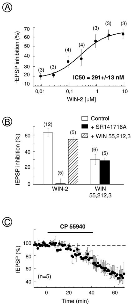
Figure 3. Pharmacological characterization of the CB1-mediated inhibition. A , Dose–response curve for the CB1 agonist WIN-2. The EC_{50} for WIN-2 was 291 \pm 13 nm. Each point is expressed as the percentage of inhibition of basal evoked transmission, and the error bar represents the SEM. B , WIN 55,212,3 ( 10 \mu\text{M} ), an enantiomer of WIN-2 inactive at CB1 binding sites, caused a small but significant fEPSP inhibition that, contrary to the WIN-2-induced inhibition, was not reversed by SR 141716A ( 10 \mu\text{M} ; black bar). WIN-2-mediated fEPSP reduction was additive to the WIN 55,212,3 effect (hatched bar). These data are in agreement with the idea that WIN-2 at concentrations up to 10 \mu\text{M} is selective for CB1 receptors. C , The cannabinoid agonist CP 55940 ( 2 \mu\text{M} ; n = 5 ), which is not structurally related to WIN-2, also inhibited fEPSP.
