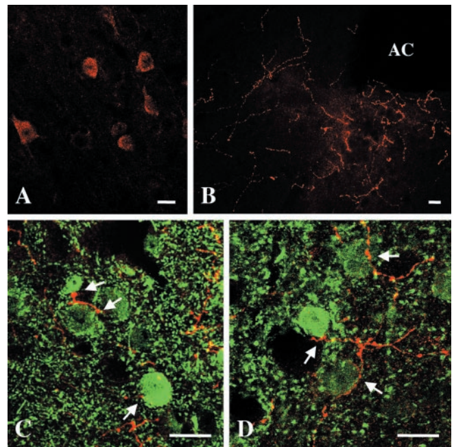
Figure 1. Localization of CB1 receptors in the prelimbic cortex and the nucleus accumbens. Confocal images of single- or double-immunostained sections. A , Single immunostaining for CB1 shows that intense labeling is associated with perikarya located in the prelimbic cortex. B , CB1 labeling was also associated with large varicose axonal fibers that extend throughout the core of the NAc surrounding the anterior commissure. C , D , Double immunostaining for both CB1 (red) and GABA (green) shows that, within the NAc, CB1-IS fibers form terminal (arrows in C ) or en passant (arrows in D ) synaptic-like contacts with GABA-IS perikarya. AC, Anterior commissure. Scale bars, 25 \mu\text{m} .
