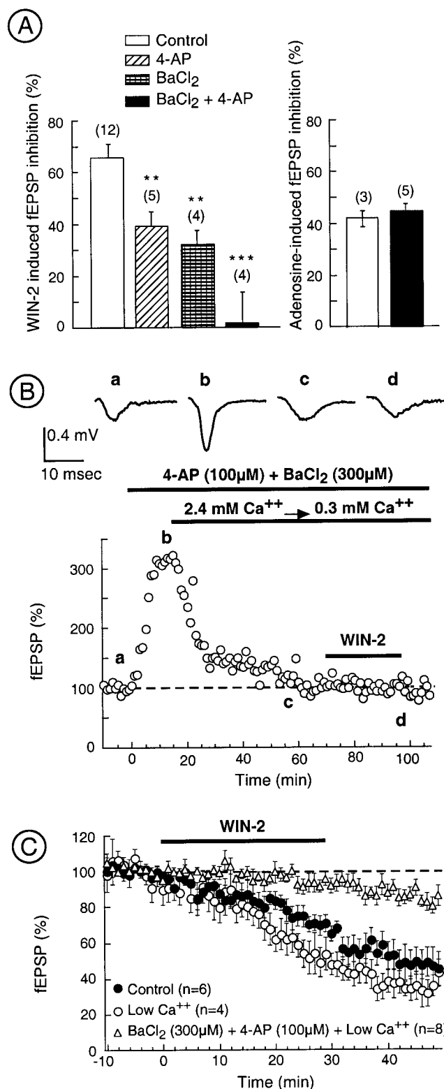
Figure 7. Effects of K + channels blockade on the CB1-induced inhibition of glutamatergic synaptic transmission in the NAc. A , In standard ACSF (2.4 mM CaCl 2 ; white bar), 4-AP (100 μM; hatched bar), and BaCl 2 (300 μM; dotted bar) reduced the WIN-2-induced fEPSP inhibition. WIN-2 reduced fEPSP by 39.1 ± 5.5% ( n = 5; p = 0.015) and 32.3 ± 9.4% ( n = 4; p = 0.029) in the presence of 4-AP and BaCl 2 , respectively, compared with 65.6 ± 5.4% ( n = 12) in control. When added together, 4-AP and BaCl 2 (black bar) completely prevented the WIN-2 (10 μM) inhibition (1.7 ± 11%; n = 4; p = 0.002). In contrast, the adenosine (200 μM; white bar)-induced inhibition was not affected by pretreatment with 4-AP and
