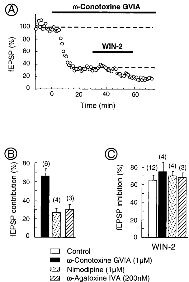
Figure 6. The WIN-2-induced inhibition does not require N-, L-, or P/Q-type Ca 2+ channels modulation. A , Typical experiment in which the slice was perfused with 1 \mu M \omega -Conotoxin-GVIA, which blocked \sim 60\% of the fEPSP. It is clear that the fraction of synaptic transmission insensitive to \omega -Conotoxin-GVIA was still sensitive to the CB1 agonist WIN-2 (10 \mu M). B , Summary of all of the experiments performed as above with specific blockers of N-type ( \omega -conotoxin-GVIA, 1 \mu M), L-type (nimodipine, 1 \mu M); and P/Q-type ( \omega -Agatoxin-IVA, 200 nM) voltage-sensitive Ca 2+ channels. The histogram of the maximum inhibitions caused by perfusion of selective agents reveals how the different types of voltage-sensitive Ca 2+ channels contribute to the evoked release of glutamate in the NAc. C , Histogram of the maximum 10 \mu M WIN-2-mediated inhibition in the presence of Ca 2+ channel inhibitors. All experiments were performed as in A .
