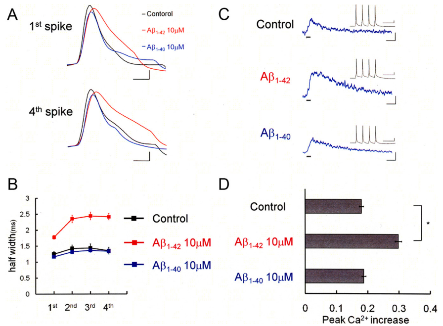
Figure 1. Intracellular infusion of A \beta_{1-42} broadens spike width and augmented Ca ^{2+} influx in rat neocortical pyramidal neurons. A , Action potentials evoked in neurons injected with A \beta . The first and fourth action potentials in spike trains are shown. Recordings taken from the control neuron (black), an A \beta_{1-42} -injected neuron (red), and an A \beta_{1-40} -injected neuron (blue) are superimposed to clarify the spike broadening in A \beta_{1-42} -injected neurons. Calibration: 1 ms, 20 mV. B , Average spike half-width in four-spike trains, showing that injection of A \beta_{1-42} ( 10 \mu\text{M} ; red square; n = 6 ), but not that of A \beta_{1-40} ( 10 \mu\text{M} ; blue square; n = 6 ), broadened spike width compared with control neurons (black square; n = 6 ). C , Ca ^{2+} increases induced by four-spike trains (inset) in control neurons and in neurons injected with 10 \mu\text{M} A \beta_{1-42} or 10 \mu\text{M} A \beta_{1-40} . Calibration: 500 ms, -0.1 \Delta F_{380}/F_{360} . Inset, Specimen recording of a spike train at 18 Hz that was used for the shown Ca ^{2+} measurements. The timing of each spike is shown by a small black triangle below the trace. Note the difference in time scale. Calibration: 100 ms, 20 mV. D , Summary diagram demonstrating average Ca ^{2+} increases. Injection of A \beta_{1-42} enhanced spike-induced Ca ^{2+} increases. * p < 0.0001 .
