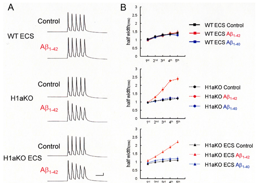
Figure 7. Blocking effects of ECS on A \beta_{1-42} was absent in H1aKO mice. A , ECS counteracts A \beta_{1-42} -mediated spike broadening in wild-type mice (WT ECS) but not in H1aKO mice (H1aKO, H1aKO ECS). Calibration: 20 ms, 20 mV. B , Averaged spike half-width during spike trains (black, Control; red, A \beta_{1-42} ) with ECS in wild mice (top), without ECS in H1aKO mice (middle), and with ECS in H1aKO mice (bottom). Each point is an average of four to six trials.
