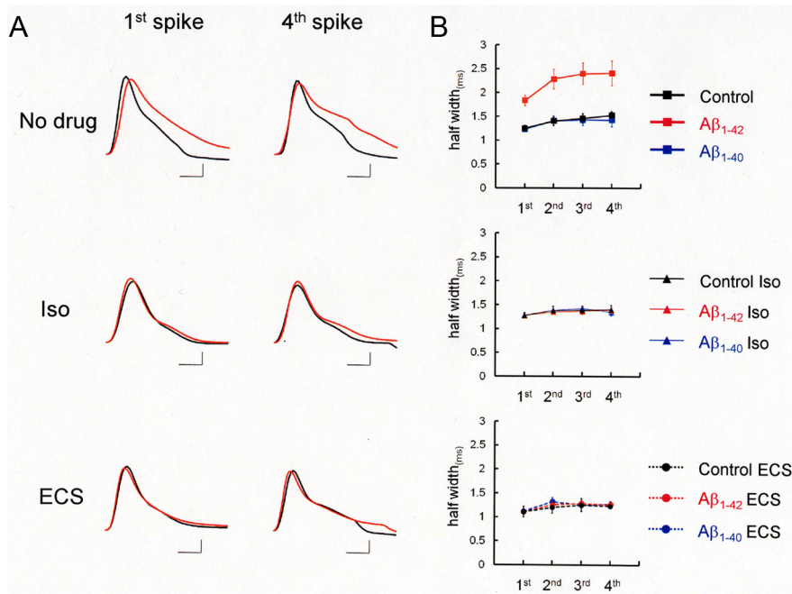
Figure 5. ECS blocked A \beta_{1-42} -mediated suppression of BK channels in rat neocortical neurons. A , First and fourth spike in spike trains under the application of the BK channel opener isopimaric acid (Iso; 10 \mu M) or after ECS, in a control neuron (black) and an A \beta_{1-42} -injected neuron (red). The same spike broadening as observed with fura-2 was confirmed without fura-2 in patch pipettes (Fig. 1). Note differences to the same extent in spike width between cells with (red line) and without intracellular A \beta_{1-42} (black line, No drug). Both isopimaric acid and ECS prevented A \beta_{1-42} from broadening spike width. Calibration: 1 ms, 20 mV. B , Averaged spike half-width during four-spike trains (black, Control; red, A \beta_{1-42} ; blue, A \beta_{1-40} ) with No drug (top), with Iso (middle), and after ECS (bottom). Each point is based on an average over four to eight trials.
