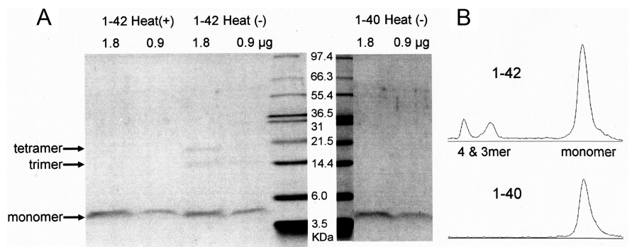
Figure 2. Detection of A \beta_{1-42} oligomers in the pipette solution. A , A \beta_{1-42} and A \beta_{1-40} were taken from the pipette solution and prepared for SDS-PAGE. Two different amounts ( 1.8 and 0.9 \mu\text{g} ) were used. Samples were heated [Heat(+)] before loading for controls or left without heating [Heat(-)]. Based on the molecular-weight marker, the positions for monomer, trimer, and tetramer were determined. For A \beta_{1-42} only, in addition to the monomer, bands are also positive at the trimer and tetramer positions, albeit to much lesser extents than the monomer band [ 1-42 Heat(-), 1.8 \mu\text{g} ]. B , Band density profiles. By applying the Plot Lanes function (ImageJ software) to scanned gel images, density profiles were drawn for the lanes loaded with unheated A \beta_{1-42} [ 1-42 Heat(-), 1.8 \mu\text{g} ] and A \beta_{1-40} [ 1-40 Heat(-), 1.8 \mu\text{g} ]. Relative optical density was plotted in an arbitrary unit for each lane. The top-to-bottom direction in the lane is reflected to the left-to-right direction in this diagram. Compared with the peak density for the monomer band, those for trimer and tetramer were much lower for A \beta_{1-42} and undetectable for A \beta_{1-40} .
