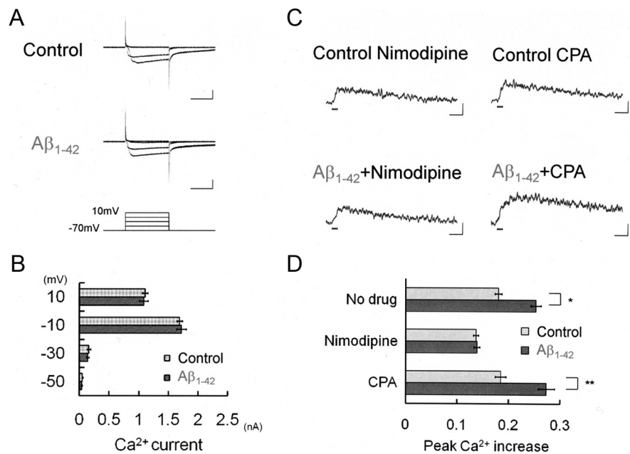
Figure 4. Failure of intracellular A \beta_{1-42} to directly modulate Ca ^{2+} channels. A , Ca ^{2+} currents with 1 \mu M A \beta_{1-42} ( n = 10 ) or without A \beta_{1-42} (Control; n = 7 ) infused. Calibration: 100 ms, 1 nA. B , The peak amplitude of Ca ^{2+} current (elicited by voltage steps to -50 , -30 , -10 , and 10 mV) was compared. A \beta_{1-42} infusion has no effects on Ca ^{2+} currents. C , The voltage-dependent Ca ^{2+} channel blocker nimodipine (20 \mu M; Control, n = 5 ; A \beta_{1-42} , n = 5 ), but not the Ca ^{2+} store depletor CPA (30 \mu M; Control, n = 6 ; A \beta_{1-42} , n = 5 ), abolishes the enhancement of spike-induced Ca ^{2+} increase by A \beta_{1-42} . Ca ^{2+} channel activation becomes stronger with A \beta_{1-42} , rather indirectly, because of BK channel suppression by A \beta_{1-42} (Fig. 3). Calibration: 500 ms, -0.1 \Delta F_{380}/F_{360} . D , Peak amplitude of spike-induced Ca ^{2+} increases in the presence of nimodipine or CPA, indicating that Ca ^{2+} release channels are not involved at all. * p < 0.001 ; ** p < 0.01 .
