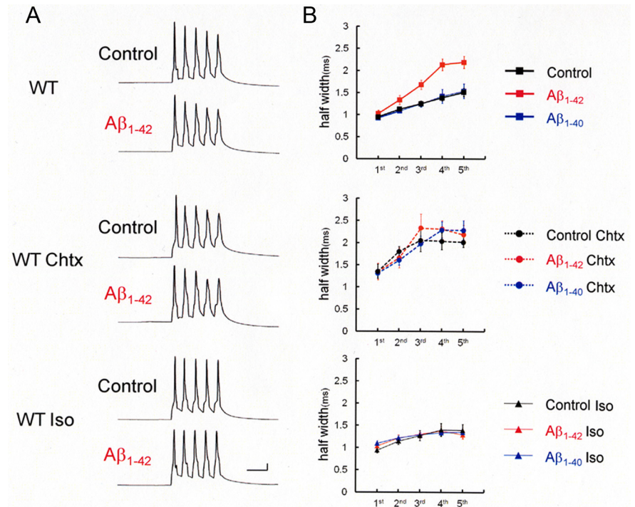
Figure 6. A \beta_{1-42} injection into neurons in slices obtained from wild mice caused spike broadening. A , Recordings of spike trains induced by brief current injections at 100 Hz into neurons in slices obtained from wild mice. With A \beta_{1-42} injected intracellularly, spike half-widths in later spikes were significantly larger than in no-A \beta controls. Charybdotoxin mimics and occludes and Iso blocks the actions of A \beta_{1-42} , indicating that spike broadening is caused by A \beta_{1-42} -mediated blockade of BK channels. Calibration: 20 ms, 20 mV. B , Averaged spike half-width during the five-spoke train (black, Control; red, A \beta_{1-42} ; blue, A \beta_{1-40} ) with no drug (top), with Ctx (middle), and with Iso (bottom). Each point is an average of four to six trials.
