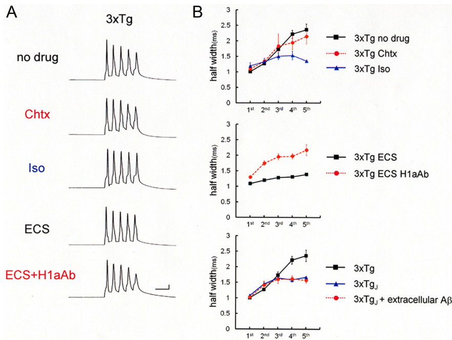
Figure 8. Spike broadening in 3xTg neurons. A , Recordings of spike trains in the 3xTg mice at 4 months of age, exhibiting spike broadening. The top recording shows spike broadening in the naive condition (no drug, n = 6 ). The addition of charybdotoxin failed to broaden spikes further ( n = 4 ), exhibiting occlusion of the blocker effect. Iso blocked the spike broadening ( n = 4 ). The bottom two recordings show spike trains in neurons from 3xTg mice after ECS. ECS on 3xTg mice blocked the spike broadening, which was cancelled out by injection of anti-Homer1a antibody ( 0.4 \mu\text{g/ml} ; ECS, n = 6 vs ECS + H1aAb, n = 7 ). Calibration: 20 ms, 20 mV. B , Averaged spike width in 3xTg cells. Top, Spike half-width is shown for naive 3xTg neurons (No drug; black square), those with BK channel blockade (Chtx; red circle), and those with Iso (blue triangle). Middle, Averaged spike half-width after ECS with H1aAb (ECS + H1aAb; red circle) or without (ECS; black square). Bottom, Spike half-width recorded in neurons from juvenile 3xTg (16–18 d old; 3xTg J ), in which intracellular A \beta has not yet been accumulated. Spike width was smaller in 3xTg J neurons (3xTg J ; blue triangle) than in 3xTg neurons (3xTg; black square) and remained at a range comparable with that in wild controls. Extracellular application of A \beta_{1-42} ( 1 \mu\text{M} ) to 3xTg J cells failed to broaden spikes (3xTg J + extracellular A \beta ; red circle).
