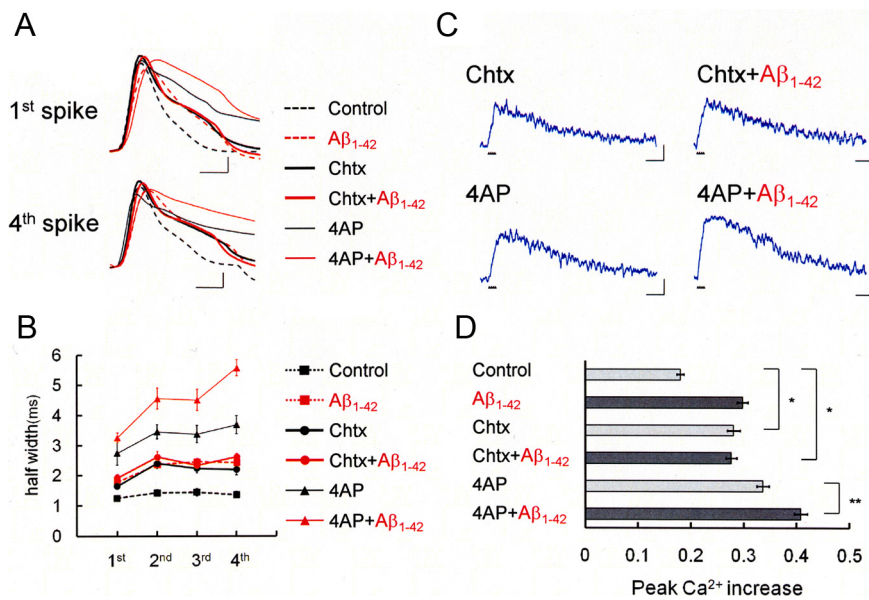
Figure 3. Intracellular A \beta_{1-42} enlarges spike width by suppressing BK channels, thereby increasing spike-induced Ca 2+ entry. A , First and fourth action potentials during spike trains after application of the BK channel blocker Chtx (50 nM) or the A-type K + channel blocker 4-AP (5 mM) in a control cell (Chtx: thick black trace, n = 7 ; 4-AP: thin black trace, n = 5 ) and an A \beta_{1-42} -injected cell (Chtx + A \beta_{1-42} : thick red trace, n = 4 ; 4-AP + A \beta_{1-42} : thin red trace, n = 4 ). The action potentials in the control cell (black dashed trace) and A \beta_{1-42} -injected cell (red dashed trace) shown in Figure 1 are superimposed. Calibration: 1 ms, 20 mV. B , Averaged spike half-width during four-spike trains with no blocker (black square, Control; red square, A \beta_{1-42} ), with charybdotoxin (black circle, Control; red circle, A \beta_{1-42} ) and with 4-AP (black triangle, Control; red triangle, A \beta_{1-42} ). C , Spike-induced Ca 2+ increase under application of charybdotoxin or 4-AP in control or A \beta_{1-42} -injected neurons. Calibration: 500 ms, -0.1 \Delta F_{380}/F_{360} . D , Summary diagram demonstrating average Ca 2+ increases in the control, charybdotoxin, and 4-AP groups, each with and without A \beta_{1-42} . In B and D , charybdotoxin, but not 4-AP, mimicked and occluded the effect of A \beta_{1-42} . * p < 0.0001 , ** p < 0.01 .
