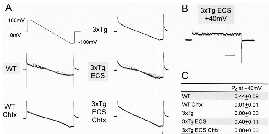
Figure 9. Recovery of single BK current by ECS in 3xTg mice. A , A ramp-voltage command from +100 to –100 mV (top left) induces single BK currents in wild mice (WT; n = 6 ) and 3xTg mice after ECS (3xTg ECS; n = 5 ), but not in 3xTg mice without ECS (3xTg; n = 6 ). These single currents were blocked by Chtx ( n = 5 ; 3xTg ECS Chtx, n = 4 ). The dotted lines indicate the open or closed states. Calibration: 200 ms, 10 pA. B , Single BK currents were confirmed by a rectangle voltage command from 0 to +40 mV in 3xTg mice after ECS. This voltage step was used, since the open probability hereby was found close to ~50%. Calibration: 200 ms, 5 pA. C , Open probability (P o ) based on recordings with step commands to +40 mV. Each point is an average of four to six trials.
