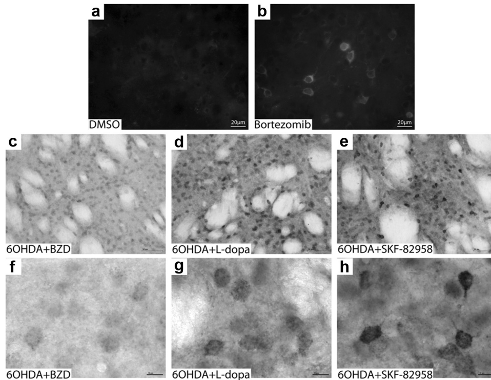
Figure 4. In vivo GFP reporter accumulation in 6-OHDA Ub G76V -GFP transgenic mice demonstrates functional proteasome catalytic activity impairment in medium spiny neurons after L-DOPA. a, b , Immunofluorescent labeling of striatal sections of Ub G76V -GFP mice demonstrates Ub G76V -GFP positive neurons after bortezomib treatment ( b ) as compared with DMSO control ( a ). c–h , Immunoperoxidase detection of GFP immunoreactivity (Avidin–biotin DAB Nickel technique) in striatal medium spiny neurons of unilateral 6-OHDA-lesioned mice (scale bars, 50 μm). Control mice (benserazide only) ( c, f ); L-DOPA-treated 6-OHDA-lesioned mice with AIMs ( d, g ); SKF-82958-treated 6-OHDA-lesioned mice ( e, h ). Medium spiny neurons of L-DOPA-treated 6-OHDA-lesioned mice ( d, g ) display a strong accumulation of GFP compared with benserazide group ( c, f ). More intense accumulation was observed when mice were treated with D1R full agonist SKF-82958 ( e, h ).
