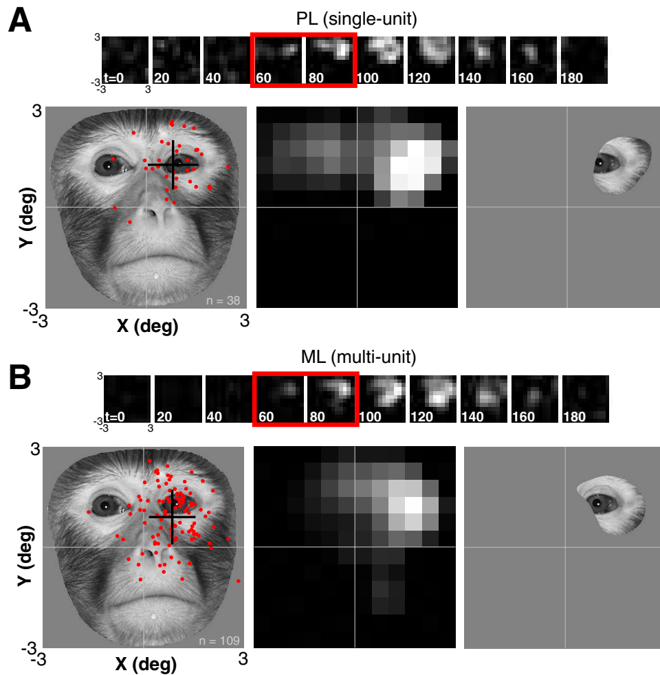
Figure 6. Reverse correlation mapping for single units and in ML. A , Preferred face regions of single units recorded in PL were centered near the contralateral eye (black crosshair; compare to Fig. 3A; same plotting conventions used). B , Preferred face regions of individual multiunit sites recorded in ML (compare to Fig. 3A; same plotting conventions used).
