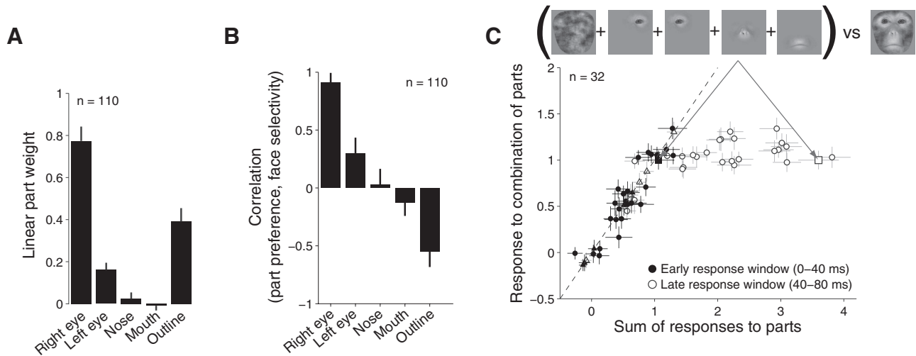
Figure 8. Linear contribution of face outline and contralateral eye. A , The linear contribution of each human-segmented face part (right eye, left eye, nose, or mouth) when testing all possible combinations ( 2^4 = 16 total images) in the context of a face outline. B , Correlation of part preference (i.e., w_{\text{part}}/\sum |w_i| ) with face selectivity index. C , The median response of the population to all possible part combinations where the presence of the outline was also varied ( 2^5 - 1 = 31 total images) plotted against the sum of the responses to the parts (vertical bars, SD of responses across the sites tested; horizontal bars, SD of the sum of parts responses across the sites tested; triangles, single-part responses; square symbols, whole-face response vs the sum of the responses to the five parts). Prior to averaging across sites, the responses for each site were rescaled by the average response to the whole face.
