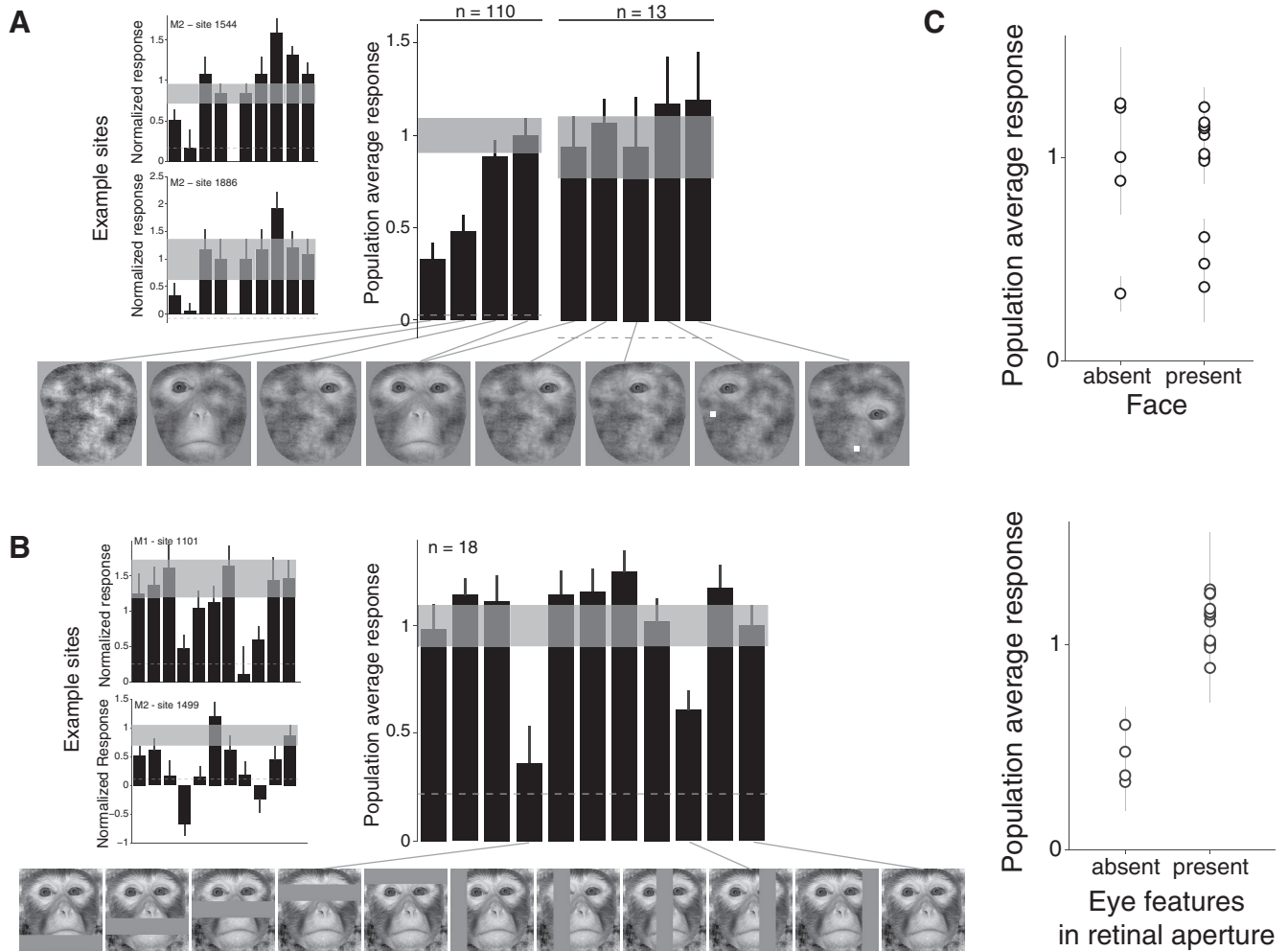
Figure 10. Images predicted to drive early responses in PL. A , Left, Responses to images containing some or all of the face parts in the context of the face outline. Right, The outline-relative position of the eye could be varied across a wide range and still drive early responses in PL sites. The white square indicates the fixation point when not on the center of the image. Insets, Responses of two example sites to the same images. B , Reduced early responses for faces were found when a horizontal or vertical bar occluded the contralateral eye. Insets, Responses of two example sites to horizontally or vertically occluded faces. C , Top, PL responses were poorly predicted by whether a face was present or absent (face considered present if at least half of the face is visible and absent otherwise). Bottom, PL responses were relatively well predicted by whether eye-like features were in the upper contralateral visual field. Raw average of individual site responses shown in A and B were rescaled by the median response to the whole face. Dashed lines indicate the median response to nonface objects.
