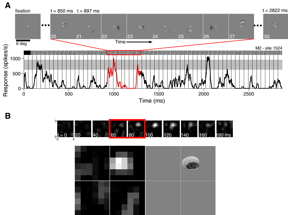
Figure 2. Face reverse correlation mapping. A , Gaussian windowed face fragments were presented in rapid succession (every 47 ms or 21 Hz) while the monkey fixated a central fixation square (white) for up to 3 s. The example site (bottom row) responded strongly during frames when the interior of the eye was present. (Notice the strong response to the first and last frame in the red highlighted region. Frames are offset by the site's overall latency, 76 ms, to aid visual alignment with responses. The gray region denotes the response level in the screen set to the whole face). B , Top, Reverse correlation analysis was performed to determine the linear response weighting of 0.5 \times 0.5^\circ regions of the face in 20 ms response bins. Z-scored weights are plotted. Bottom left, The spatial kernels in the early response window (60–100 ms; red rectangle) were averaged to generate the weighting map for the early response. Bottom right, The image fragment corresponding to the weighting region at half-height was extracted.
