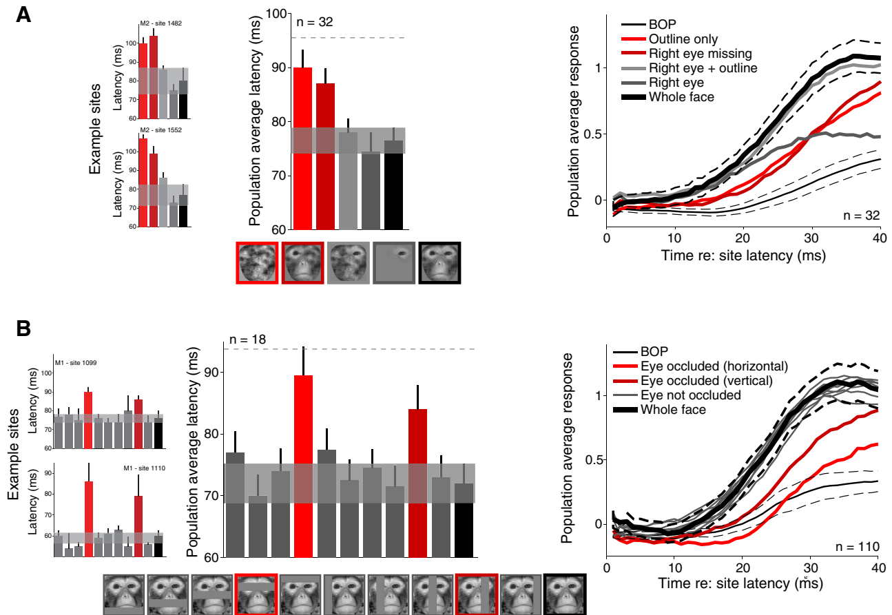
Figure 12. Response latency when the eye region was absent or occluded. A , Simply presenting the right eye (dark gray) but not the outline (light red) led to a response latency as short as for the whole face (black). Removing the right eye delayed responses even when all of the other face parts were present (dark red). Insets, Response latencies in two example sites for the same set of images. B , Latency increased when occluding the contralateral eye region using a horizontal or vertical bar (red) but not when occluding other regions of the face (gray). Insets, Response latencies of two example sites to horizontally and vertically occluded images. A, B , Right, Population-averaged PSTHs shown rescaled by the median response to the whole face at 100 ms. Individual site PSTHs were aligned by their minimum latency to faces, bodies, objects, or places before averaging.
