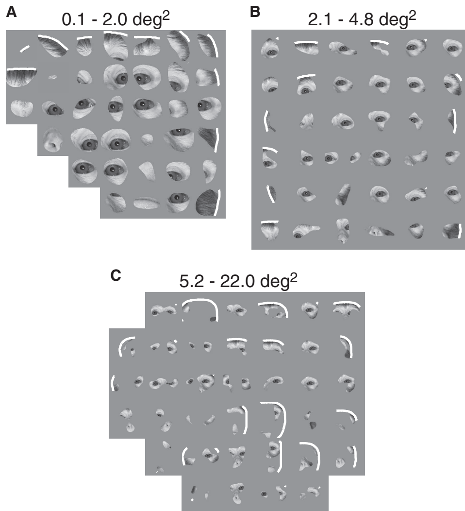
Figure 4. Preferred face fragments of individual sites in PL. Face fragments (50% regions) for individual sites are grouped based on their size and ordered by their relative position for ease of display. A, B , For sites whose preferred regions were small or intermediate in size, the right eye was the most common feature. C , Larger regions tended to encompass both eyes. For sites with multiple half-height regions, only the two largest are plotted, and most sites had only one half-height region ( A, B ). White outlines mark the edge of the face outline for reference, and features without a white outline lie toward the interior of the face.
