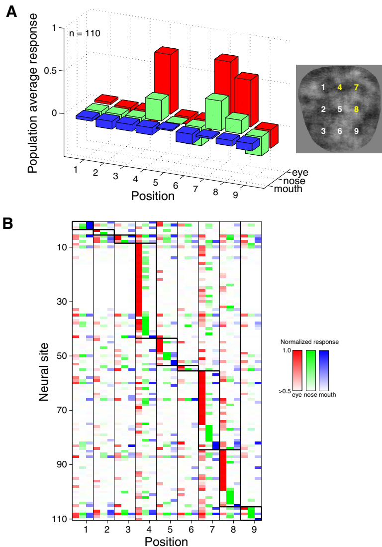
Figure 9. Effect of retinal position on responses to face parts. A , Population-average responses to the face parts (eye, nose, and mouth) tested at nine possible positions on the face outline (the response to the outline alone was subtracted, and responses were normalized by the median outline-subtracted response to the whole face). B , Bottom, Color histogram showing the responses of individual sites to the eye, nose, and mouth presented at nine different positions. Sites are ordered by their position preference (black boxes) followed by their feature preference at the preferred position (i.e., eye-selective sites appear first followed by nose- and then mouth-selective sites). Responses are thresholded at half-maximum (see color legend).
