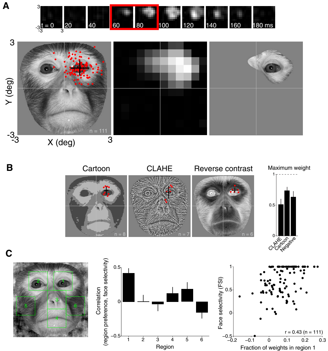
Figure 3. Preference for the eye region in PL. A , In a majority of sites, weights in the early response window (60–100 ms; red outline) were centered in the top contralateral quadrant (left; dots reflect centroid of preferred region for individual sites; crosshair reflects mean and SD of x, y centers across sites; white dot is the center of the preferred region from the example site in Fig. 2). The corresponding face fragment (50% contour of the population response that was obtained by averaging z-scored weights across sites) was centered on the eye (middle, right). B , The eye region was the most strongly weighted part of the face in cartoon (left), CLAHE (middle), and reversed-contrast faces (right). Peak response weights for these manipulated images are plotted relative to the median of the maximum weights for the original face image (far right). C , The face selectivity index was correlated with the fraction of weights in the eye region in reverse correlation maps (right) but was not correlated with the fraction of weights in other regions of the face (middle). Six nonoverlapping regions across the face were tested (left).
