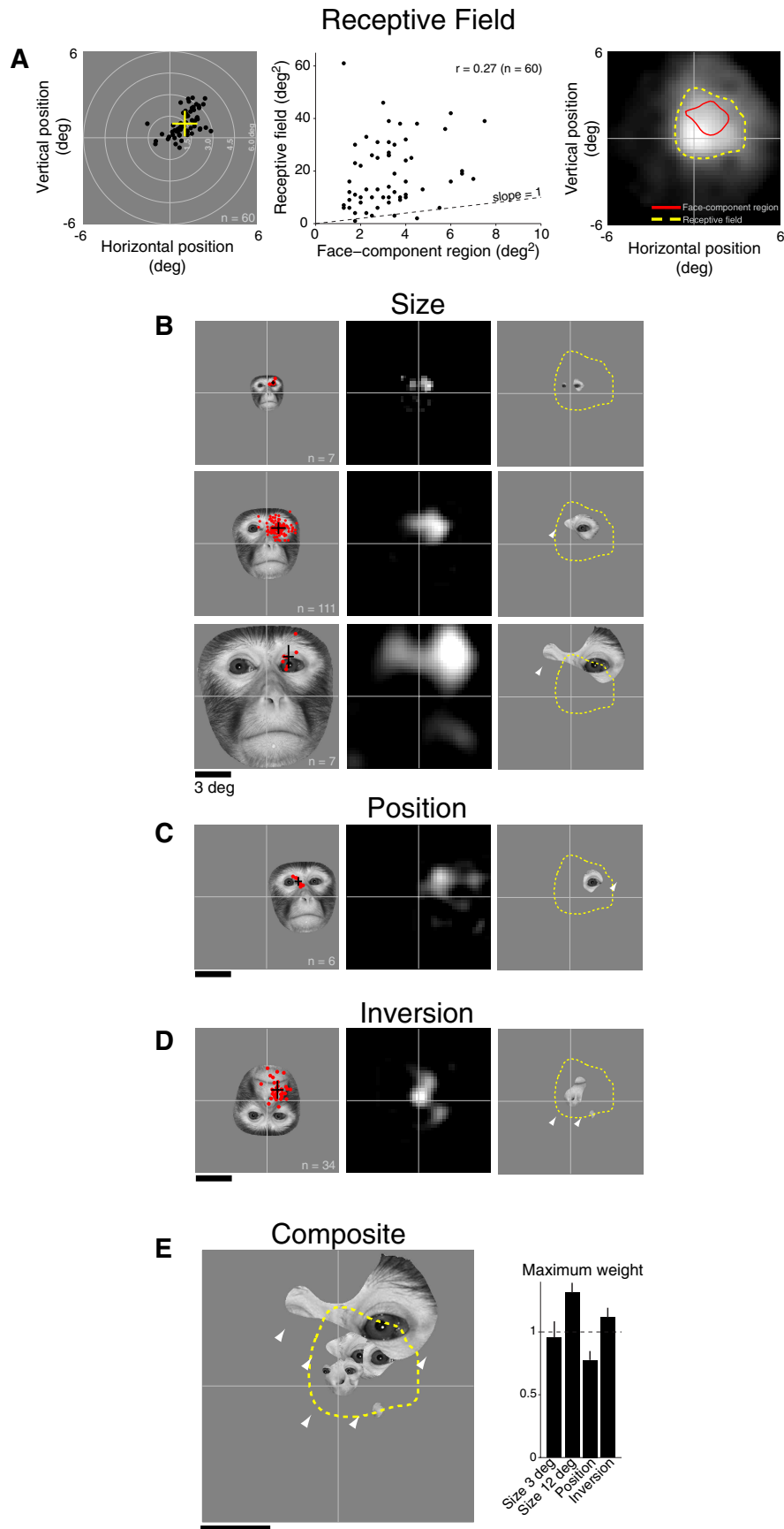
Figure 7. Size and position tolerance of eye selectivity in PL. A , Left, Retinal RFs in PL (black dots reflect receptive field centers of individual sites; crosshair reflects mean and SD of centers across the population). Middle, The size of RFs was only weakly predictive of the size of the preferred face components of individual sites, and retinal RFs tended to be larger than preferred face components. Right, The population retinal RF (yellow outline) was larger in size than the population-averaged face-component region (red). B , The eye region was preferred ( Figure legend continues. )
