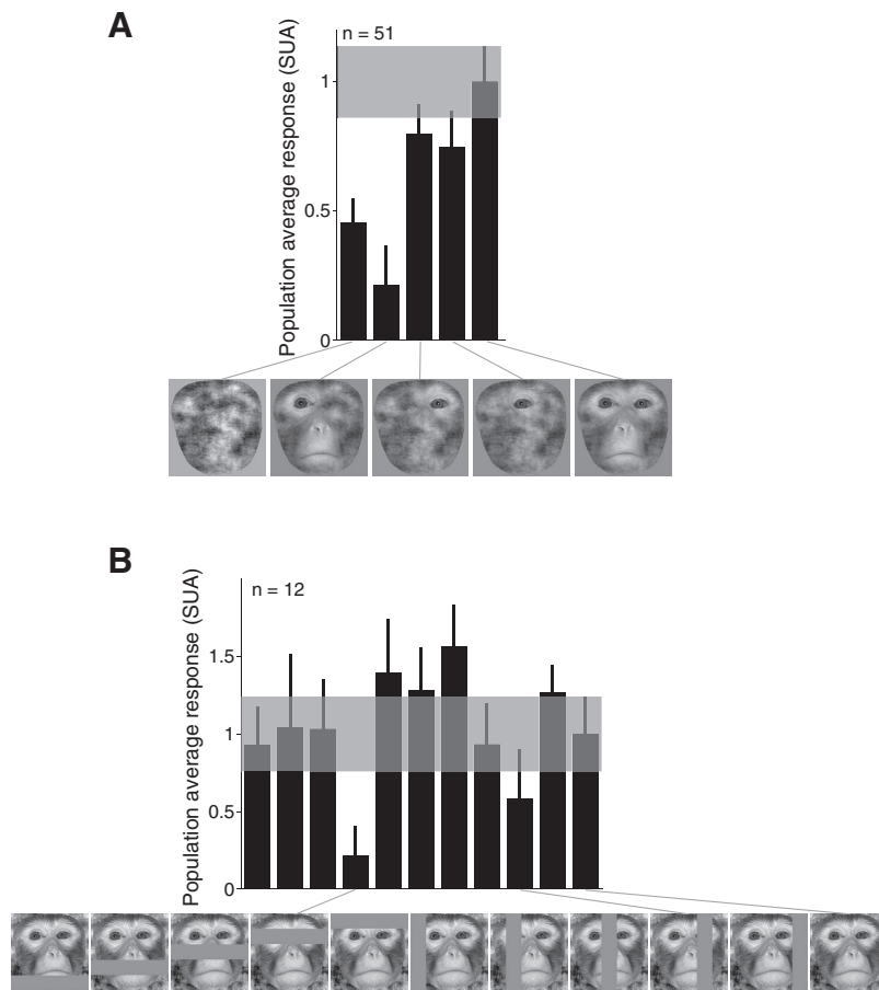
Figure 11. Responses of single units when the eye region was absent or occluded. A , Single-unit responses were highest when an eye was present in the upper, contralateral field and were strongly reduced when the contralateral eye was absent, even though all other face parts were present. B , Single-unit responses were strongly reduced when both eyes were occluded and weakly reduced when the contralateral eye was occluded.
