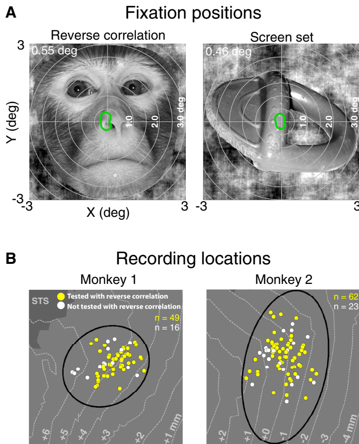
Figure 5. Eye fixations and recording locations for reverse correlation mapping. A , Fixation positions during testing with the general screen set and during reverse correlation mapping. Contours represent 90th percentile of fixation positions along each radial direction (sampled at 15° intervals). Polar grids are plotted at 0.5° spacing. B , Recording maps in each monkey are shown for the subset of sites characterized using reverse correlation. Sites are labeled based on whether they were tested (yellow) or not tested (white). Site positions were projected to the boundary between gray and white matter before flattening of the cortical patch (black circle, approximate projection to the surface of physiologically defined boundary of PL at its widest extent in 3D; dashed contour lines are projected Horsely–Clarke AP coordinates; STS, superior temporal sulcus; similar plotting conventions as in Fig. 1A).
