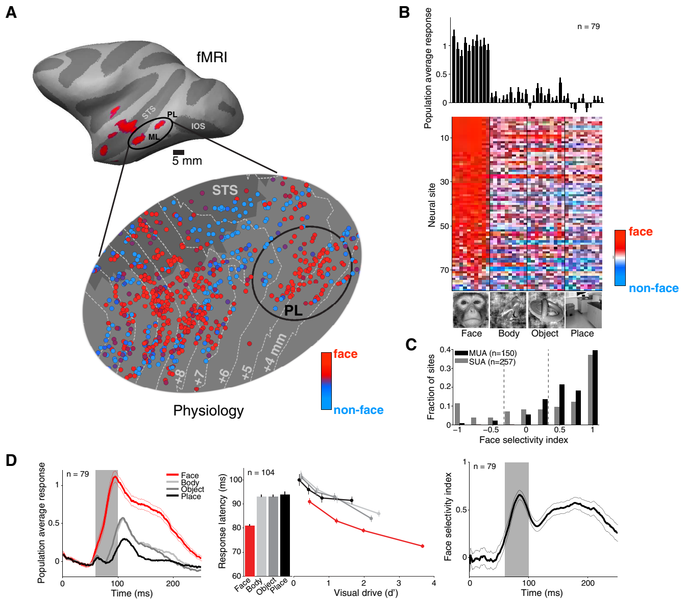
Figure 1. Face selectivity in PL. A , Top, PL is the most posterior patch in the inferior temporal lobe demonstrating face selectivity under fMRI; ML is also labeled for reference. Data are shown for Monkey 1. fMRI in Monkey 2 also revealed the posterior face patch bilaterally. Bottom, Physiological map of multiunit recordings in IT reveals a posterior cluster of face-selective sites corresponding to PL as identified in fMRI (sites colored by neuronal response d' for faces vs the mean across bodies, objects, and places; site positions and physiologically defined boundary of PL, at its widest extent in 3D, were projected in native 3D space to the 2D boundary between gray and white matter before flattening of the 2D cortical patch; dashed contour lines are projected Horsely–Clarke AP coordinates). STS, Superior temporal sulcus; IOS, inferior occipital sulcus. B , Responses of sites in PL to the standard screen set of faces, bodies, objects, and places (10 exemplars per category). Top, Individual site responses were averaged to generate the population response, which is shown rescaled by the average response to faces. Bottom, Sites were first rescaled by their maximum image response and rank-ordered according to their mean response across face exemplars. C , Comparison of multiunit and single-unit face selectivity distributions (FSI; see Materials and Methods). Antipreferring face sites (FSI < 0) were more common in single units than in multiunits. D , Left, Face images drove a strong early response compared to bodies, objects, and places (gray box denotes early response window of 60–100 ms; population-average response shown rescaled by the median response to the whole face at 100 ms). Middle, PL responses to faces had significantly shorter latencies than responses to bodies, objects, and places at all levels of visual drive (measured as d' of response above baseline; this analysis required between-site comparisons of latencies for responses with matched visual drive). Given that higher firing rates lead to shorter latencies slope, approximately -5 ms per unit of d' , this analysis demonstrates shorter latencies for faces compared to other object categories independent of overall visual drive. Right, The FSI peaked within the first 40 ms of the response.
