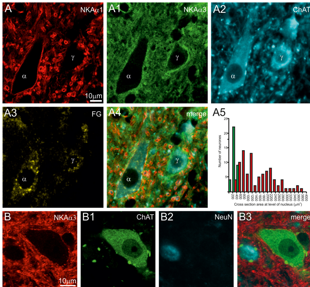
Figure 4. NKA \alpha 3 is found in small \gamma -motoneurons, while larger \alpha -motoneurons express NKA \alpha 1. Immunoreactivity for NKA \alpha 1 and NKA \alpha 3 reveals two distinct populations of motoneurons within the ventral horn (A–A5). Neurons were confirmed as motoneurons through the expression of ChAT (A2) and retrograde labeling from the periphery with Fluorogold (A3). Measuring the area of the motoneurons expressing either NKA \alpha 1 (A5, red bars) or NKA \alpha 3 (A5, green bars) reveals two distinct populations of neurons based upon size. The likelihood of the small motoneurons immunoreactive for NKA \alpha 3 being \gamma -motoneurons was strengthened through the absence of NeuN within these neurons (B–B3).
