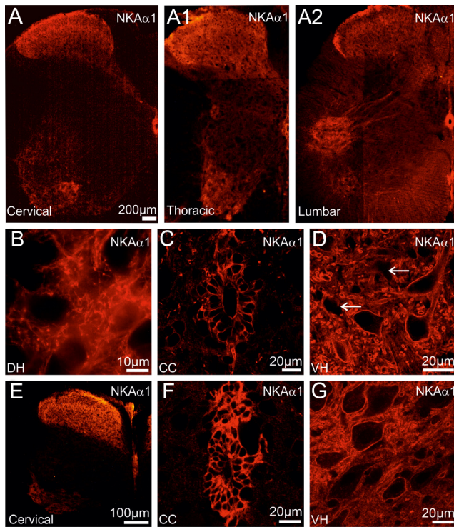
Figure 2. NKA \alpha 1 immunoreactivity is observed within motoneurons in the spinal cord. NKA \alpha 1 immunoreactivity displays the same pattern across all levels of the spinal cord ( A–A2 ). Within the superficial laminae of the dorsal horn, fine fibers and puncta are immunoreactive for NKA \alpha 1 ( B ). In lamina X, close to the central canal, NKA \alpha 1-IR is absent from neurons and is expressed strongly in the membranes of the ependymal cells surrounding the central canal ( C ). Within the ventral horn, NKA \alpha 1-IR is only found in the membranes of large presumed \alpha -motoneurons, with smaller NKA \alpha 1-IR-devoid neurons indicated with arrows ( D ). The staining pattern observed at postnatal day 6 ( E–G ) closely resembles that observed in the adult. DH, Dorsal horn; VH, ventral horn; CC, central canal.
