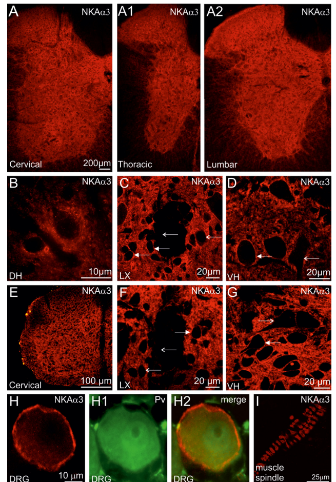
Figure 3. NKA \alpha 3 immunoreactive neurons can be observed throughout the spinal cord and in a subpopulation of DRG neurons. NKA \alpha 3 immunoreactivity is more ubiquitous than NKA \alpha 1-IR, with immunoreactivity throughout the neuropil at all levels of the spinal cord ( A–A2 ). Within the deeper laminae of the dorsal horn, NKA \alpha 3-IR is observed in punctate structures ( B ). Within lamina X close to the central canal, NKA \alpha 3-IR is observed throughout the neuropil, with some immunoreactive neurons visible ( C ). In the ventral horn of the spinal cord, NKA \alpha 3-IR can be found in close proximity to neurons. The smaller neurons appear to have more NKA \alpha 3-IR enriched around their membranes ( D ). At postnatal day 6 ( E–G ), the pattern of immunoreactivity appears identical to that observed in the adult. In dorsal root ganglia, NKA \alpha 3-IR was observed within a proportion of the parvalbumin expressing large neurons ( H–H2 ). Consistent with this, NKA \alpha 3-IR could also be observed within the membranes of muscle spindles ( I ). Examples of NKA \alpha 3-IR and NKA \alpha 3-IN neurons are marked with closed and open arrows, respectively. DH, Dorsal horn; VH, ventral horn; LX, lamina X; DRG, dorsal root ganglion.
