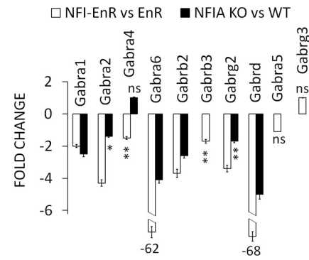
Figure 2. NFI controls GABA A receptor switch gene expression. qRT-PCR assays of GABA A receptor subunit genes that undergo developmental changes in gene expression during CGN maturation. Changes were assessed in 6 DIV CGN cultures transduced on 0 DIV with NFI/EnR or EnR lentivirus, and in P15 Nfia (+/+) (WT) and (-/-) (KO) cerebella. Larger fold changes for the Gabra6 and Gabrd genes are shown numerically below the bars. p < 0.001 except * p < 0.05 , ** p < 0.01 ; ns, no significant difference. Data are representative of three independent experiments.
