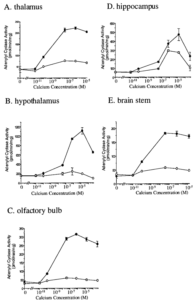
Figure 3. Brain-region specific AC activity in WT and AC8 KO mice. Calcium-stimulated AC activity determinations from freshly excised thalamus ( A ), hypothalamus ( B ), olfactory bulb ( C ), hippocampus ( D ), and brainstem ( E ) from WT (closed circles; n = 5 ) or AC8 KO (open circles; n = 5 ) mice are displayed. Nearly all AC8 KO brain regions, with the exception of the hippocampus, demonstrated profound deficiency in the ability to generate cAMP in response to Ca^{2+} .
