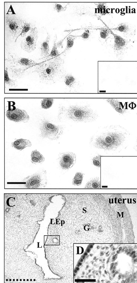
Figure 4. Expression of ER- \alpha and ER- \beta in microglia and macrophages. Direct-light photomicrographs of ER- \alpha immunoreactivity in microglia ( A ) and macrophages (M \Phi ; B ). The small insets correspond to a parallel immunostaining in which the primary antibody was omitted. C , ER- \alpha distribution in the luminal epithelium ( LEp ), gland cells ( G ), stroma ( S ), and smooth muscle structures ( M ) of rat uterus. L , Lumen. D , Magnification of the boxed area in C , showing the nuclear localization of the staining. Black bars are 40 \mu m, dashed bar is 1 mm, and bar in D is 10 \mu m. Photographs were made by using a 990 Coolpix digital photocopier, then visualized and printed using standard computer programs.
