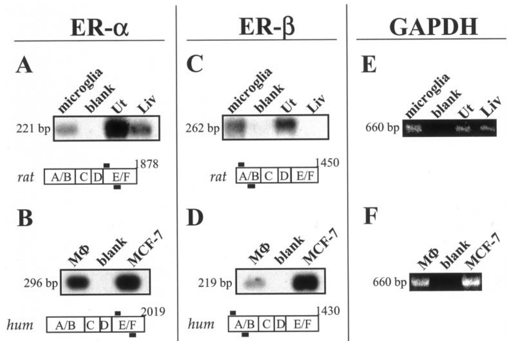
Figure 5. Expression of ER- \beta mRNA in microglia and macrophages. Microglia and macrophage (M \Phi ) ER- \alpha (A, B), ER- \beta (C, D), and GAPDH (E, F) mRNAs were assayed by RT-PCR, followed by Southern blot analysis (A–D). The annealing site of the PCR primers are reported as black boxes with the representation of the respective rat and human ( hum ) cDNAs; the length of the amplification products are reported on the left of each panel. Rat uterus ( Ut ), liver ( Liv ), MCF-7 cells, or negative controls (blank, in which microglia or macrophage RNAs were assayed without adding the RT enzyme) were also analyzed. Hybridized membranes were exposed to autoradiographic films for 1 hr (A, B) or 3 hr (C, D) at room temperature. E, F, Photographs of the GAPDH amplification products on ethidium bromide-stained gels.
