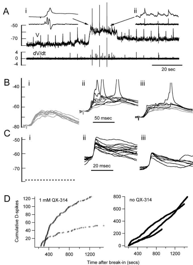
Figure 2. Voltage dependence and sensitivity to QX-314 of dendritic spikes. A , The top trace shows a continuous current-clamp recording with and without hyperpolarizing current injection with the corresponding derivatized record underneath. A stimulating pipette inserted into the superficial external plexiform layer stimulated synaptic inputs at 5 s intervals (stimulus artifacts can be seen in voltage recording but were removed from the derivatized record for clarity). The insets are expanded time base segments from portions of the continuous record, as indicated by the arrows. Inset Ai shows evoked D-spikes and an aborted action potential; inset Aii shows spontaneous D-spikes between stimuli. With hyperpolarization to about -79 mV, only three D-spikes are evoked and no spontaneous D-spikes occur. At about -60 mV, many spontaneous D-spikes occur and synaptic potentials evoke action potentials with several D-spikes. Intermediate hyperpolarization to about -72 mV produced one spontaneous D-spike and several evoked D-spikes. B , C , Segments of data extracted from another 2 min of recording from the same cell during which the membrane potential was adjusted similar to the records shown in A . Records in which no D-spikes were seen are presented in gray; those with D-spikes are black. B , Stimulation evokes only synaptic potentials at -79 mV ( Bi ); D-spikes and sometimes action potentials are evoked at -65 mV ( Bii ) or -71 mV ( Biii ) average resting membrane potential. C , Spontaneous D-spikes do not occur at -79 mV ( Ci ) resting membrane potential, as indicated by dashed line, and are seen at a lower frequency for -71 mV ( Cii ) versus -65 mV ( Ciii ). D , A cumulative count of all D-spikes shows that 1 mM QX-314 added to the pipette gradually blocks the occurrence of spontaneous D-spikes (results from 2 cells shown in left panel). Without QX-314, D-spikes are produced at a constant rate as illustrated by data from three other cells (right). The vertical axes are in millivolts or volts per second for A–C .
