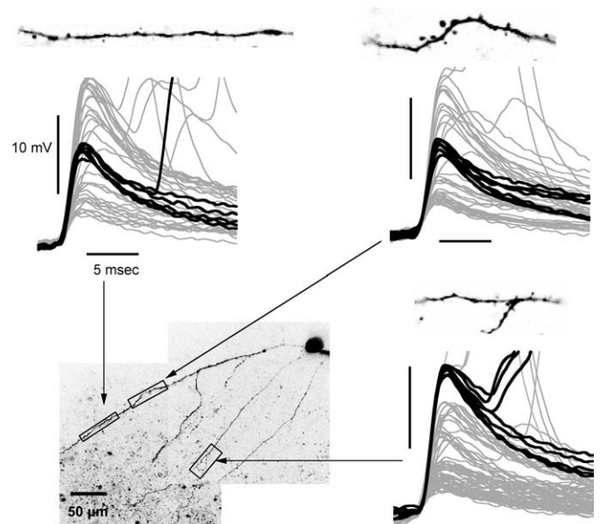
Figure 6. Ca 2+ transients associated with different electrophysiologically defined D-spikes can be localized to different branches. Each panel shows dendritic spikes from a total of 57 s of simultaneous electrophysiology and imaging. The black segments show those D-spikes that were associated with fluorescence transients and those D-spike plus APs that were associated with transients that were >150% of the size of the transients of EAPs. The gray segments indicate that either no transient was produced by a D-spike or, if an action potential was triggered from a D-spike, a transient was seen with an amplitude similar in size to that produced by EAPs. These data show that transients in the same primary dendrite were associated with D-spikes of a similar size, whereas those in a different dendrite correlated with a different class of dendritic spikes.
