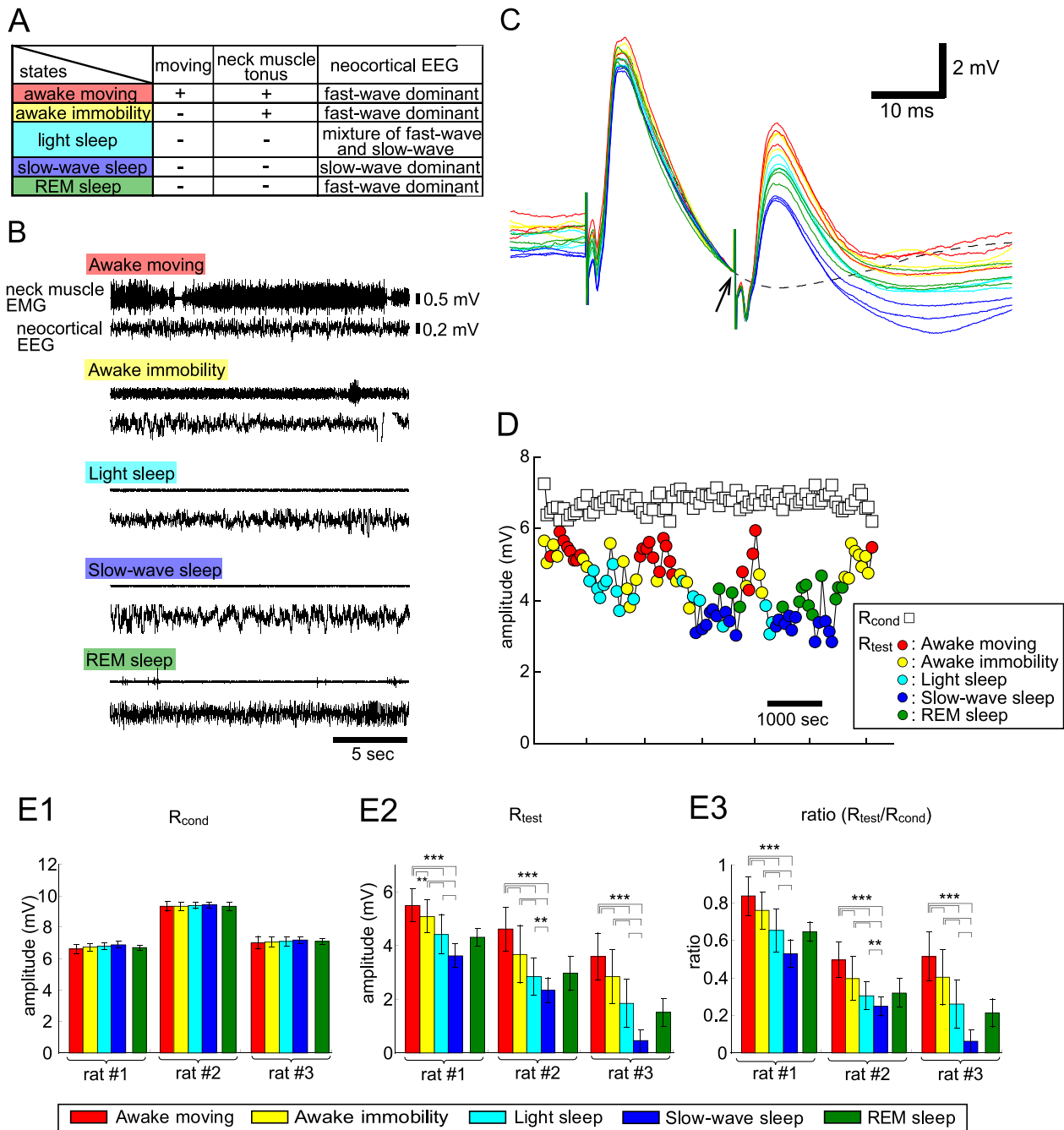
Figure 7. Behavioral state-dependent multilevel changes in the granule-to-mitral inhibition in freely behaving rats. A , We classified behavioral states into five categories on the basis of the behavior, neck muscle EMG, and neocortical EEG. B , Examples of neck muscle EMG and neocortical EEG in each behavioral state. During the awake moving and awake immobility states, we observed tonic activity in the neck muscle and high-frequency waves in the EEG. During the slow-wave sleep state, the neck muscle showed no tonus and the neocortical EEG had a slow-wave pattern. The time window of each trace is 20 s. C , Field potential responses recorded in the GCL of the OB to paired LOT stimulation in a freely behaving rat. LOT-evoked field potentials during awake moving (3 red traces), awake immobility (3 yellow traces), light sleep (3 light blue traces), slow-wave sleep (3 dark blue traces), and REM sleep (3 green traces) states are overlaid. These traces were aligned by the potential just before the test stimulus (indicated by arrow). The ISI was 20 ms. The broken black line indicates the average of 10 responses to a single LOT stimulation. Note that the amplitude of the response to the test stimulus was the smallest during the slow-wave sleep state. D , Chronological plots of the amplitude of the test response ( R_{test} ) and the conditioning response ( R_{cond} ). Paired LOT stimulation was applied once every 60 s and 100 times per day. White squares indicate R_{cond} , and colored circles indicate R_{test} . The different colors indicate behavioral states of the animal when paired LOT stimulation was applied: red, awake moving; yellow, awake immobility; light blue, light sleep; dark blue, slow-wave sleep; green, REM sleep. Note that R_{test}/R_{cond} decreases during sleep states, and is lowest during the slow-wave sleep state. E1–E3 , Quantitative comparison of the amplitude of R_{cond} ( E1 ), R_{test} ( E2 ), and R_{test}/R_{cond} ( E3 ) across distinct behavioral states (red, awake moving; yellow, awake immobility; light blue, light sleep; dark blue, slow-wave sleep; green, REM sleep; means \pm SD). The amplitude of R_{cond} did not show clear differences across behavioral states. In contrast, the amplitude of R_{test} and the ratio R_{test}/R_{cond} were significantly different across the awake moving, awake immobility, light sleep, and slow-wave sleep states (** p < 0.01 ; *** p < 0.001 , ANOVA combined with Tukey's post hoc test). The amplitude of R_{test} and the ratio R_{test}/R_{cond} did not show significant differences between the light sleep state and REM sleep state.
