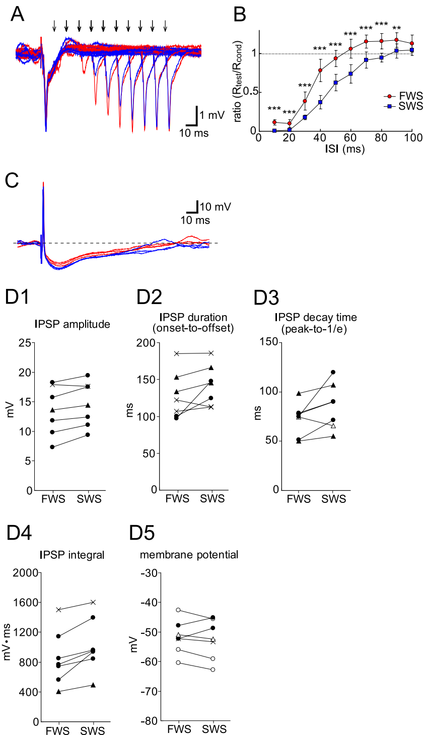
Figure 2. Granule-to-mitral inhibition is longer during SWS than during FWS in the OB of urethane-anesthetized rats. A , LOT-evoked field potentials in the EPL were recorded at various conditioning-to-test intervals from 10 to 100 ms. Arrows indicate the times of the test LOT stimulations. Artifacts of the test LOT stimulation were eliminated. Recordings during FWS are shown by red traces and those during SWS by blue traces. B , The ratio of R_{test} and R_{cond} ( R_{test}/R_{cond} , mean \pm SD) was plotted against ISI. Means and SD were calculated from 9 to 20 recordings at each ISI and in each state in one animal (** p < 0.01 ; *** p < 0.001 , two-tailed t tests with Bonferroni's correction). The suppression of the test LOT-evoked response by the conditioning LOT stimulation was stronger and longer during SWS than during FWS. C , An intracellular recording from a mitral cell showing an antidromic spike and a long-lasting IPSP induced by the LOT stimulation. LOT-evoked IPSPs during FWS (3 red traces) were overlaid with those during SWS (3 blue traces). The IPSP tended to be larger and longer during SWS than during FWS despite the same resting membrane potential. D1–D5 , Averaged IPSP amplitude ( D1 ), IPSP duration (onset-to-offset; D2 ), IPSP decay time (peak-to-1/e; D3 ), IPSP integral ( D4 ), and resting membrane potential ( D5 ) in individual cells. Filled circles and filled triangles in D1–D5 indicate that the value was significantly larger during SWS than during FWS (filled circles, p < 0.01 ; filled triangles, p < 0.05 ; two-tailed t test). Open circles and open triangles in D3 and D5 indicate that the value was significantly smaller during SWS than during FWS (open circles, p < 0.01 ; open triangles, p < 0.05 ; two-tailed t test). Cross marks indicate that the value was not significantly different between the two states.
