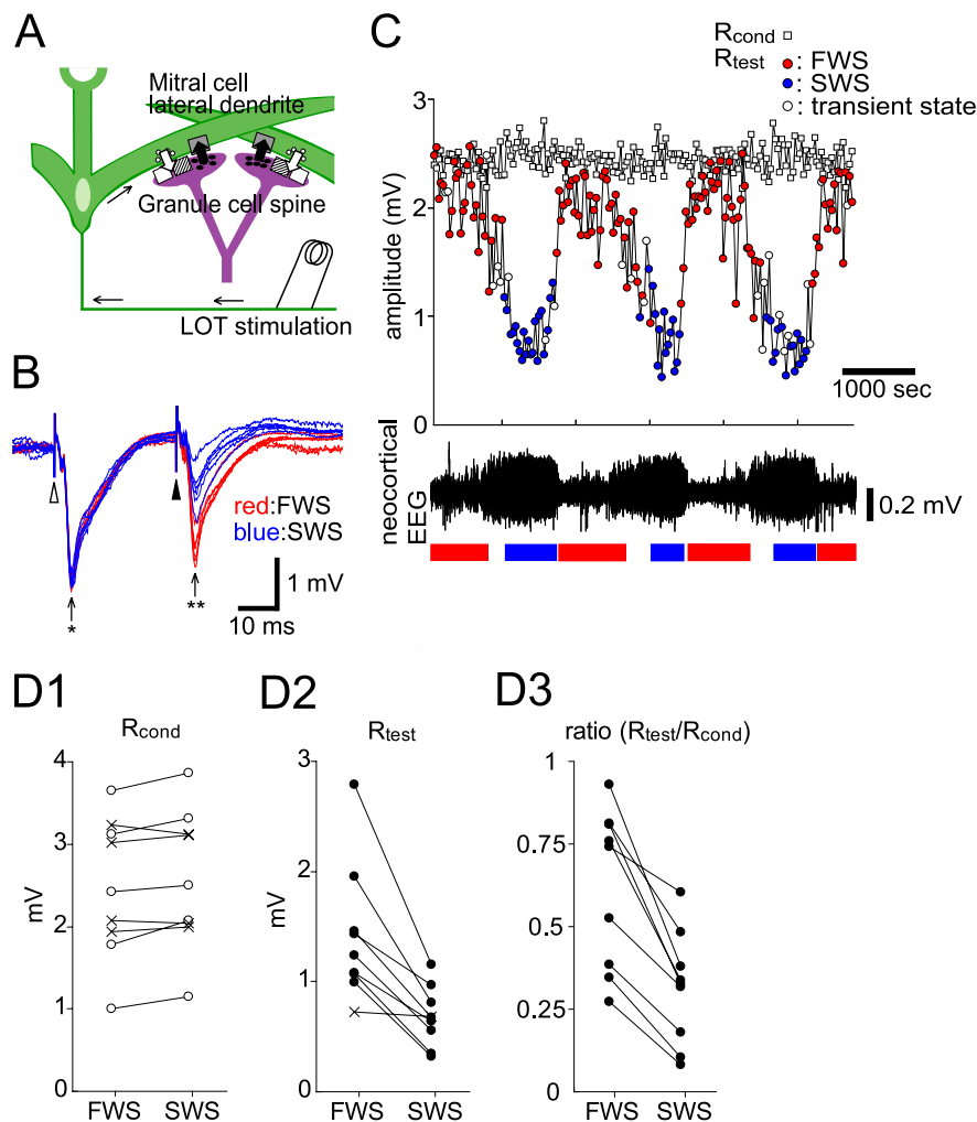
Figure 1. Granule-to-mitral inhibition is stronger during SWS than during FWS in the OB of urethane-anesthetized rats. A , A schematic diagram of dendrodendritic reciprocal synapses between mitral cell lateral dendrites and granule cell spines. Open arrows, glutamatergic excitatory input; closed arrows, GABAergic inhibitory input; white square, AMPA receptor; shaded square, NMDA receptor; gray square, GABA A receptor. B , Field potential responses in the EPL evoked by paired LOT stimulation. The ISI was 30 ms. Six traces obtained during the fast-wave state (red traces, FWS) and slow-wave state (blue traces, SWS) are overlaid. Responses to the conditioning stimulus (an arrow with asterisk) showed only small changes with behavioral state, whereas responses to the test stimulus (an arrow with two asterisks) changed dramatically between FWS and SWS. C , Chronological plots of the amplitudes of responses to the conditioning LOT stimulation ( R_{\text{cond}} ; open squares) and to the test LOT stimulation ( R_{\text{test}} ; circles). The colors of the circles indicate the brain state of the animal when paired LOT stimulation was applied. Red, FWS; blue, SWS; white, transient state. The bottom trace indicates the neocortical EEG. Under urethane anesthesia, the neocortical EEG typically shows a periodic alternation between FWS and SWS. The periods of typical FWS and slow-wave state (SWS) by blue bars. D1–D3 , Averaged amplitudes of R_{\text{cond}} ( D1 ), R_{\text{test}} ( D2 ), and their ratio ( R_{\text{test}}/R_{\text{cond}} ; D3 ) in individual animals. The ISI was 30 ms. Each connected pair of marks represents the data from a single animal. The open circles in D1 indicate that R_{\text{cond}} was significantly larger during SWS than during FWS ( p < 0.01 , two-tailed t test). The closed circles in D2 and D3 indicate that R_{\text{test}} and the ratio R_{\text{test}}/R_{\text{cond}} were significantly smaller during SWS than during FWS, respectively ( p < 0.01 , two-tailed t test). Cross marks indicate that the values were not significantly different between the two states.
