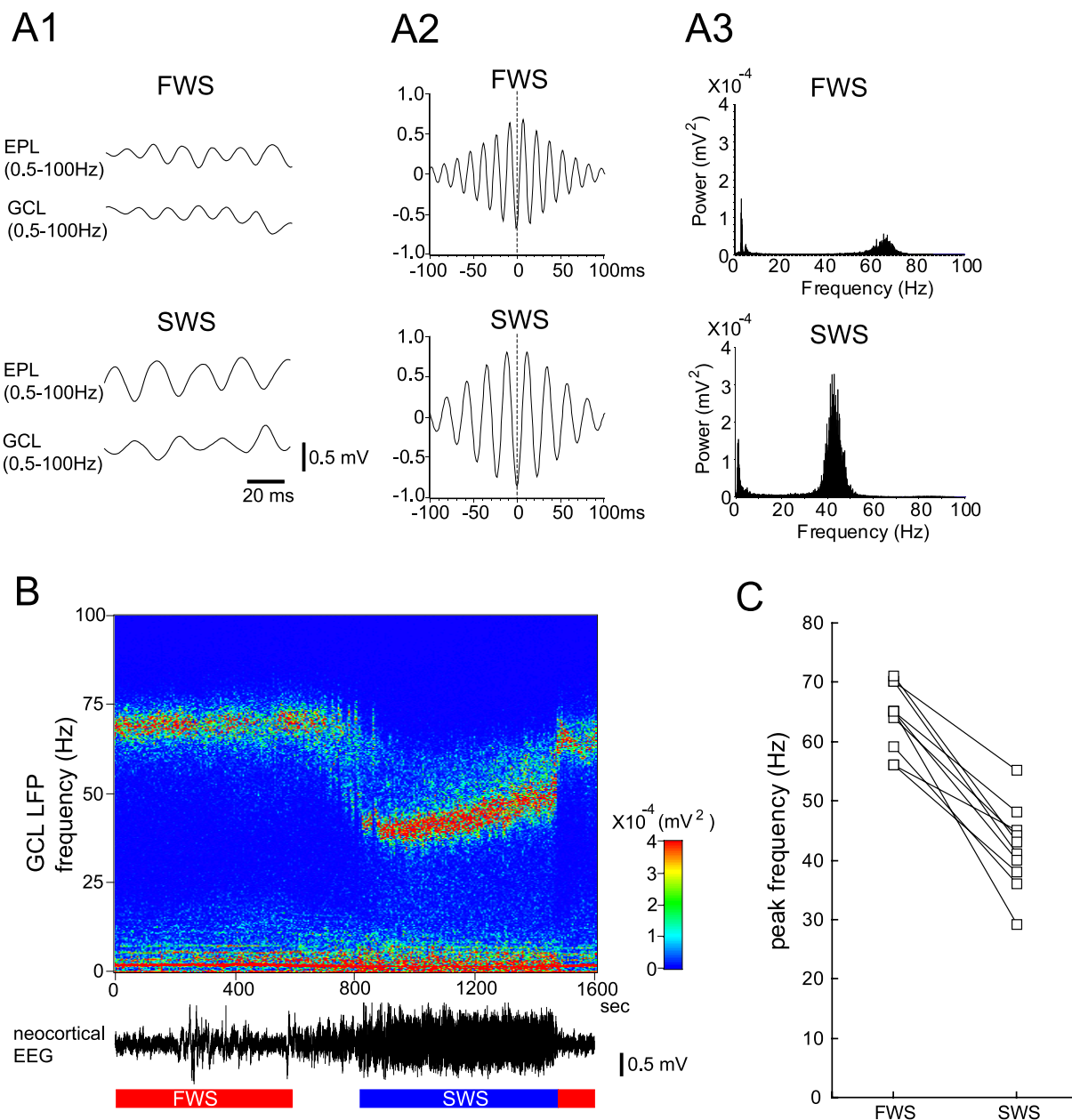
Figure 5. State-dependent change in spontaneous OLFP in the OB of urethane-anesthetized rats. A1 , Simultaneous recordings of OLFPs in the EPL (top trace) and GCL (bottom trace). The oscillation frequency of the OLFP was higher during FWS than during SWS. A2 , Cross-correlograms of OLFP recorded in the EPL and GCL during FWS (top graph; sampled for 200 s, filtered at 20–100 Hz) and during SWS (bottom graph; 200 s, 20–100 Hz). The dotted line indicates time 0. Note that the OLFPs in the EPL and in the GCL are negatively correlated. A3 , Power spectrum of the OLFP recorded in the EPL during FWS (top graph; sampled for 200 s) and during SWS (bottom graph; 200 s). B , The frequency of OLFP shifted in synchrony with the shift of brain states between FWS and SWS. OLFPs in the GCL were recorded continuously, and the power spectrum during each 5 s was calculated. This pseudocolor display of the spectrogram chronologically represents the intensity of power at each frequency. The magnitude of the power at each frequency is shown by color (right inset). x -Axis, Time (bin, 5 s); y -axis, frequency (bin, 0.24 Hz). The bottom trace indicates the neocortical EEG. C , Summary plot of the state-dependent change of OLFP peak frequency in the GCL in each animal ( n = 10 ).
