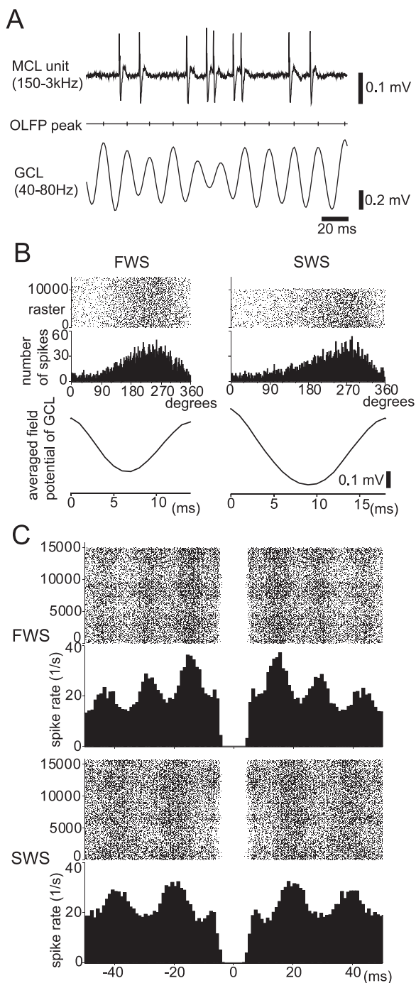
Figure 6. State-dependent change in the oscillatory spike discharges of mitral cells. A , Simultaneous recordings of mitral cell spike activity (top trace) and OLFPs in the GCL (bottom trace) during the spontaneous respiration of room air. As a reference for the phase histogram of mitral cell firing in B , the positive peaks of OLFP are noted (middle trace). B , Raster plots of spike discharges (top traces) and corresponding histograms (phase histogram, middle) are shown in relation to the phase of the OLFP (bottom trace, one averaged cycle of the OLFP). Both during FWS (left) and during SWS (right), this mitral cell fired mostly in phase with the OLFP. Note that the duration of one cycle of the oscillation is longer during SWS than during FWS. C , Spike autocorrelation plots of the spike discharges of a mitral cell during FWS (recorded for 800 s) and during SWS (800 s). The highest peak of the autocorrelation plot is located at 15 ms (67 Hz) during FWS and at 18 ms (56 Hz) during SWS.
