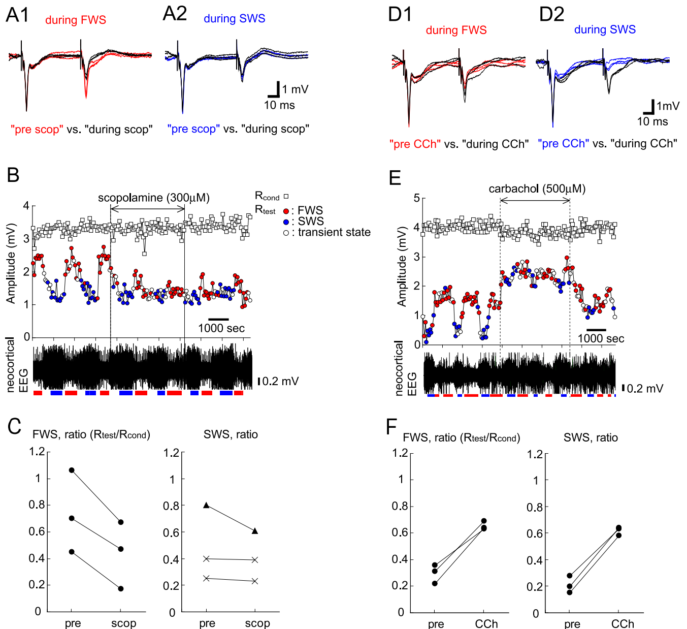
Figure 4. Cholinergic input regulates granule-to-mitral inhibition. A1 , Field potential responses in the EPL evoked by paired LOT stimulation during FWS before (3 red traces) and during (3 black traces) perfusion with scopolamine (muscarinic acetylcholine receptors antagonist, 300 \mu\text{M} ) are overlaid. The ISI was 50 ms. Note that R_{\text{test}} showed a large amount decrease during scopolamine perfusion. A2 , Field potential responses to paired LOT stimulation during SWS before (3 blue traces) and during (3 black traces) scopolamine perfusion are overlaid. B , Chronological plots of R_{\text{cond}} (squares) and R_{\text{test}} (circles) to paired LOT stimulation during ACSF perfusion on the dorsal surface of the OB. The colors of the circles indicate the brain state: red, FWS; blue, SWS; white, transient state. Scopolamine perfusion decreased R_{\text{test}} during FWS to the level of R_{\text{test}} during SWS, indicating that granule-to-mitral inhibition is regulated by muscarinic acetylcholine receptors. The bottom trace indicates the neocortical EEG. Red bar, FWS; blue bar, SWS. C , Summary plot of the averaged ratio ( R_{\text{test}}/R_{\text{cond}} ) of paired LOT stimulation before and during scopolamine perfusion ( n = 3 ). Filled circles, p < 0.01 ; filled triangles, p < 0.05 ; cross marks, no significant difference; two-tailed t test. D1 , Field potential responses to paired LOT stimulation during FWS before (3 red traces) and during (3 black traces) perfusion with carbachol (nonselective acetylcholine receptor agonist, 500 \mu\text{M} ) are overlaid. D2 , Field potential responses to paired LOT stimulation during SWS before (3 blue traces) and during (3 black traces) carbachol perfusion are overlaid. Note that R_{\text{test}} increased during carbachol perfusion. E , Chronological plots of R_{\text{cond}} (squares) and R_{\text{test}} (circles) to paired LOT stimulation during ACSF perfusion on the dorsal surface of the OB. Carbachol perfusion increased R_{\text{test}} during both FWS and SWS, indicating that granule-to-mitral inhibition is suppressed by cholinergic input. The bottom trace is the neocortical EEG. F , Summary plot of the averaged ratio of paired LOT stimulation before and during carbachol perfusion ( n = 3 ). Filled circles, p < 0.01 ; two-tailed t test.
