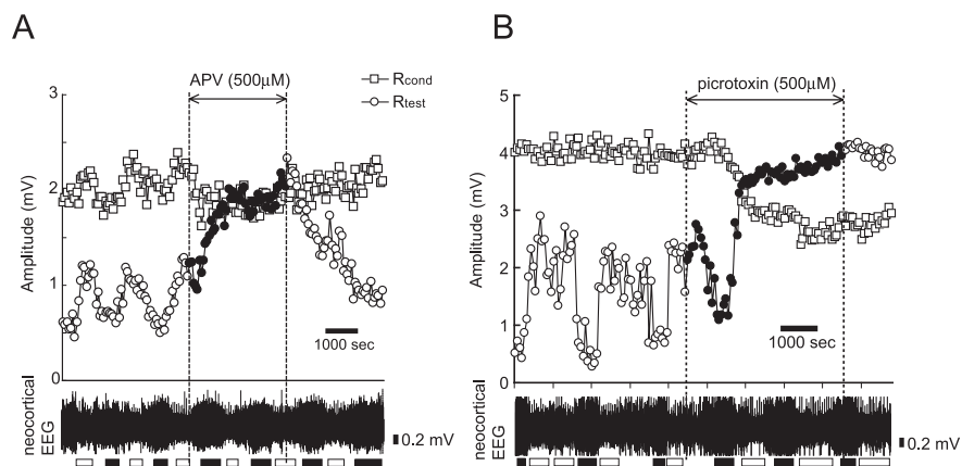
Figure 3. Pharmacological blocking of dendrodendritic synaptic interaction abolishes state-dependent change of R_{test} . A , Chronological plots of the R_{cond} (squares) and R_{test} (circles) generated by paired LOT stimulation during ACSF perfusion on the dorsal surface of the OB. The ISI was 50 ms. Black circles indicate R_{test} during perfusion with ACSF containing APV (NMDA receptor antagonist, 500 \mu M). APV perfusion increased R_{test} to the level of R_{cond} , indicating that the decrease of R_{test} is mediated by NMDA receptors. The bottom trace indicates the neocortical EEG. White bar, FWS; black bar, SWS. B , Chronological plots during perfusion with ACSF containing picrotoxin (GABA A receptor antagonist, 500 \mu M). Picrotoxin perfusion increased R_{test} , indicating that the decrease of R_{test} is mediated by GABA A receptors. The bottom trace indicates the neocortical EEG. White bar, FWS; black bar, SWS.
