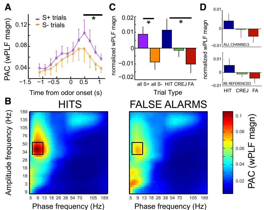
Figure 2. PAC strength: comparisons between trial types. A , Group averages (mean \pm SE over all sessions) of wPLF magnitudes in 600 ms sliding windows. Peak magnitudes occur at 500 ms after odor onset for both S+ odor-sampling periods (purple) and S− odor-sampling periods (orange). Black line indicates significant differences ( *p < 0.05 , Wilcoxon matched pairs signed rank test). B , Bispectrum of wPLF magnitude taken from the optimal PAC window ( +200 to +800 ms after odor onset), averaged across all selected channel combinations. Left, HIT trials; Right, FA trials. Black box indicates FOI \times FOI window used in further analyses. C , Group averages of mean-normalized wPLF magnitude (wPLF magnitudes for each trial type from which the common mean was subtracted; this mean was computed across all trial types) across selected channels over sessions. wPLF magnitude was calculated for the optimal PAC window ( +200 – 800 ms after odor onset) and split according to trial type. S+ trials (purple) showed significantly larger wPLF magnitude than all S− trials considered together (orange; p < 0.05 , Wilcoxon test). This difference could be unpacked into a significant difference between HIT and FA trials ( p < 0.05 ), whereas the other comparisons were not significant. Misses rarely occurred and were not further analyzed. D , As in C , but now showing mean-normalized wPLF magnitude for the control dataset that comprised session means averaged over wPLFs obtained from all channel combinations in a session ( N = 110 per session). E , As in C , but now showing mean-normalized wPLF for the re-referenced dataset.
