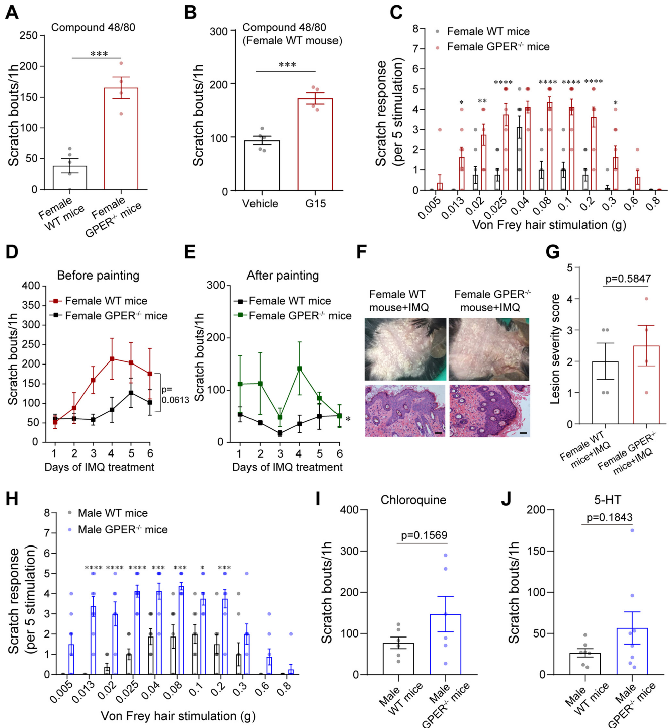
Figure 8. GPER -/- mice are hypersensitive to chemical and mechanical itch. A , Scratch bouts of female WT and GPER -/- mice induced by intradermal injection of compound 48/80 (50 \mu g/20 \mu L); n = 4 –5 mice for each group; unpaired Student's t test. p = 0.0004 , t = 6.308 , df = 7 . B , Systemic administration of G15 (0.5 mg/kg, i.p.) significantly increased scratching bouts of WT female mice induced by compound 48/80; n = 4 –5 mice; unpaired Student's t test. p = 0.0005 , t = 6.092 , df = 7 . C , Acute mechanical itch test of WT and GPER -/- female mice; n = 8 mice for each group; two-way ANOVA followed by Bonferroni's post hoc test. F_{(1,154)} = 128.1 ; 0.013 g, p = 0.0232 ; 0.02 g, p = 0.0019 ; 0.025 g, 0.08 g, 0.1 g, and 0.2 g, p < 0.0001 ; 0.3 g, p = 0.0489 . D , E , Scratching behavior of WT and GPER -/- mice on each day before ( D ) and after ( E ) painting with imiquimod cream; n = 4 mice for each group. Area under the curves (AUC) was compared using unpaired Student's t test. p = 0.0613 , t = 2.298 , df = 6 ( D ). p = 0.0287 , t = 2.863 , df = 6 ( E ). F , Photograph of the back neck and HE-stained skin of imiquimod-treated WT and GPER -/- mice. Scale bar, 50 \mu m. G , The lesion severity score of neck skin in imiquimod-treated WT and GPER -/- mice; four slides from four mice; unpaired Student's t test. p = 0.5847 , t = 0.5774 , df = 6 . H , Acute mechanical itch test of WT and GPER -/- male mice; n = 8 mice for each group; two-way ANOVA followed by Bonferroni's post hoc test. F_{(1,154)} = 140.3 ; 0.013 g, 0.02 g, and 0.025 g, p < 0.0001 ; 0.04 g, p = 0.0007 ; 0.08 g, p = 0.0001 ; 0.1 g, p = 0.0185 ; 0.2 g, p = 0.0007 . I , J , Scratch bouts of male WT and GPER -/- mice induced by intradermal injection of chloroquine ( I ; 150 \mu g/20 \mu L) and 5-HT ( J ; 10 \mu g/20 \mu L); n = 6 –8 mice for each group; unpaired Student's t test. p = 0.1569 , t = 1.531 , df = 10 ( I ); p = 0.1843 , t = 1.402 , df = 13 ( J ).
