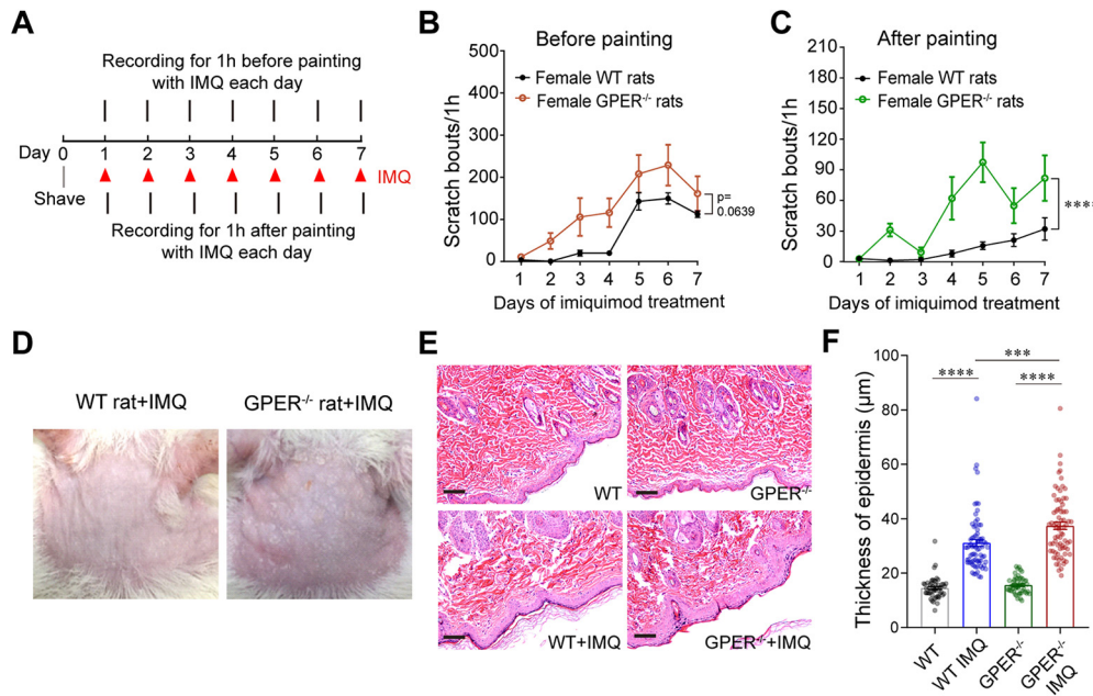
Figure 6. GPER -/- rats show increased scratching behavior than WT rats in imiquimod-induced psoriasis models. A , The timeline for imiquimod-induced psoriasis-like rat model. B , C , Scratching behavior of female WT and GPER -/- rats on each day before ( B ) and after ( C ) painting with imiquimod cream; n = 5 rats for each group; area under curves (AUC) was compared by unpaired Student's t test. t = 2.149, df = 8 ( B ). p < 0.0001, t = 8.499, df = 8 ( C ). D , Photograph of the back neck of imiquimod-treated WT and GPER -/- rats on day 8. E , HE-stained neck skin of naive and imiquimod-treated female WT and GPER -/- rats. Scale bar, 50 μm. F , The thickness of epidermis of neck skin in naive and imiquimod-treated female WT rats and female GPER -/- rats; 15 slides from three rats; one-way ANOVA and Tukey's post hoc test were used to assess statistical differences. F = 99.64; p < 0.0001 for WT versus WT IMQ and GPER -/- versus GPER -/- IMQ. p = 0.0001 for WT IMQ versus GPER -/- IMQ. IMQ, imiquimod.
