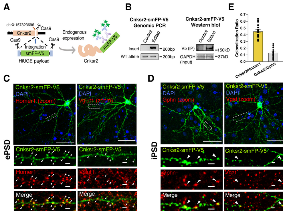
Figure 8. Cnksr2 is localized to the postsynapse. A , Schematic for HiUGE labeling of endogenous Cnksr2. B , Left, Genomic PCR detection of smFP-V5 integration at the Cnksr2 locus. Right, Western blot detection of the Cnksr2-smFP-V5 fusion protein at the expected molecular mass (~160 kDa). IP, Immunoprecipitation enrichment with V5-trap beads. C , Top, Knock-in expression of Cnksr2-smFP-V5 in cultured neurons (green) and DAPI (blue) is shown. Scale bars, 40 \mu m. Bottom left, Higher-magnification view of the boxed region shows colocalization (arrowheads) of Cnksr2-smFP-V5 immunoreactivity with Homer1 immunosignal (red). Scale bar, 2 \mu m. Bottom right, Higher-magnification view of the boxed region shows colocalization (arrowheads) of Cnksr2-smFP-V5 immunoreactivity with Vglut1 immunosignal (red). Scale bar, 2 \mu m. D , Top, Knock-in expression of Cnksr2-smFP-V5 in cultured neurons (green) and DAPI (blue). Scale bars, 40 \mu m. Bottom left, Higher-magnification view of the boxed region shows colocalization (arrowheads) of Cnksr2-smFP-V5 immunoreactivity with Gephyrin immunosignal (red). Scale bar, 2 \mu m. Bottom right, Higher-magnification view of the boxed region shows colocalization (arrowheads) of Cnksr2-smFP-V5 immunoreactivity with VGAT immunosignal (red). Scale bar, 2 \mu m. E , Graph represents colocalization ratios for Cnksr2 puncta with Homer1 (mean value 0.45) and Gephyrin (mean value 0.13). Colocalization ratios were calculated as the number of Cnksr2 puncta colocalized with Homer1 or Gephyrin divided by total number of Cnksr2 puncta. Two or three dendrites were imaged from eight or nine neurons from multiple coverslips.
