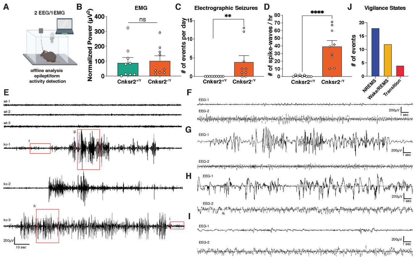
Figure 4. Cnksr2 -Y mice exhibit abnormal EEGs with epileptiform discharges. For handling-induced tonic-clonic seizure example, see also Movie 1 . A , Schematic of 2 EEG/1 EMG recording area for freely moving mice. B , Graph of EMG full-spectrum power. No significant difference in average EMG power between genotypes was observed ( p > 0.05 ; unpaired t test). Data were normalized by transforming the WT mean value into 100% and represent mean \pm SEM. C , Number of electrographic seizure events detected per day plotted for Cnksr2 +/Y and Cnksr2 -Y mice. Five WT and 5 KO mice were used for the recordings, and each mouse was recorded for 1 or 2 sessions. A total of 35 events were detected in 5 KO (7 of 9 sessions) mice, and 0 events were detected in 5 WT mice (0 of 9 sessions). **p = 0.0011 (Fisher's exact test, one-tailed). D , Number of spike-wave discharges per hour quantified for Cnksr2 +/Y and Cnksr2 -Y mice. Spike-wave complexes lasting > 1 s and separated by < 0.5 s were quantified and reported. Number of spike-wave complexes seen in EEGs were significantly increased in Cnksr2 -Y mice. ****p < 0.0001 (Mann–Whitney test). E , Representative EEG1 traces. Top, WT baseline EEGs. Bottom, Traces of electrographic seizures detected in KO mice. F , Baseline EEG-1 and EEG-2 electrode traces for ko-1 before the detected event. G , Electrographic seizures detected in EEG-1 for ko-1. H , Electrographic seizures detected in EEG-1 for ko-3. I , Baseline EEG-1 and EEG-2 electrode traces for ko-3 after the detected event. J , Identification of vigilance states in which electrographic seizure events occur in Cnksr2 -Y mouse. Nineteen events during NREMS, 12 events during awake/REMS, and 4 events during transition state between awake/REMS and NREMS were identified.
