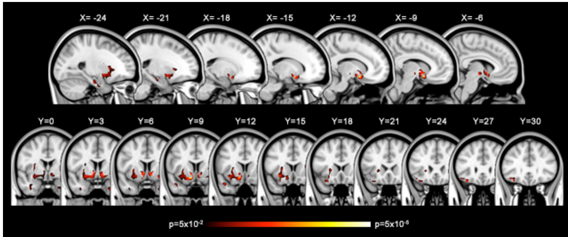
Supplementary Figure 2. Statistical map showing fractional anisotropy (FA) voxels that are negatively correlated with trait anxiety across the whole brain ( p < 0.05 , corrected for multiple comparisons over the frontal and temporal white matter tissue) in sagittal and coronal slices. Color bars indicate p -values. Voxels identified from this analysis were primarily overlapping with the voxels within an amygdala-vmPFC pathway supporting the anatomical specificity of the relationship between the identified amygdala-vmPFC pathway and trait anxiety. No significant voxels were identified outside of the a priori frontal or temporal white matter.
